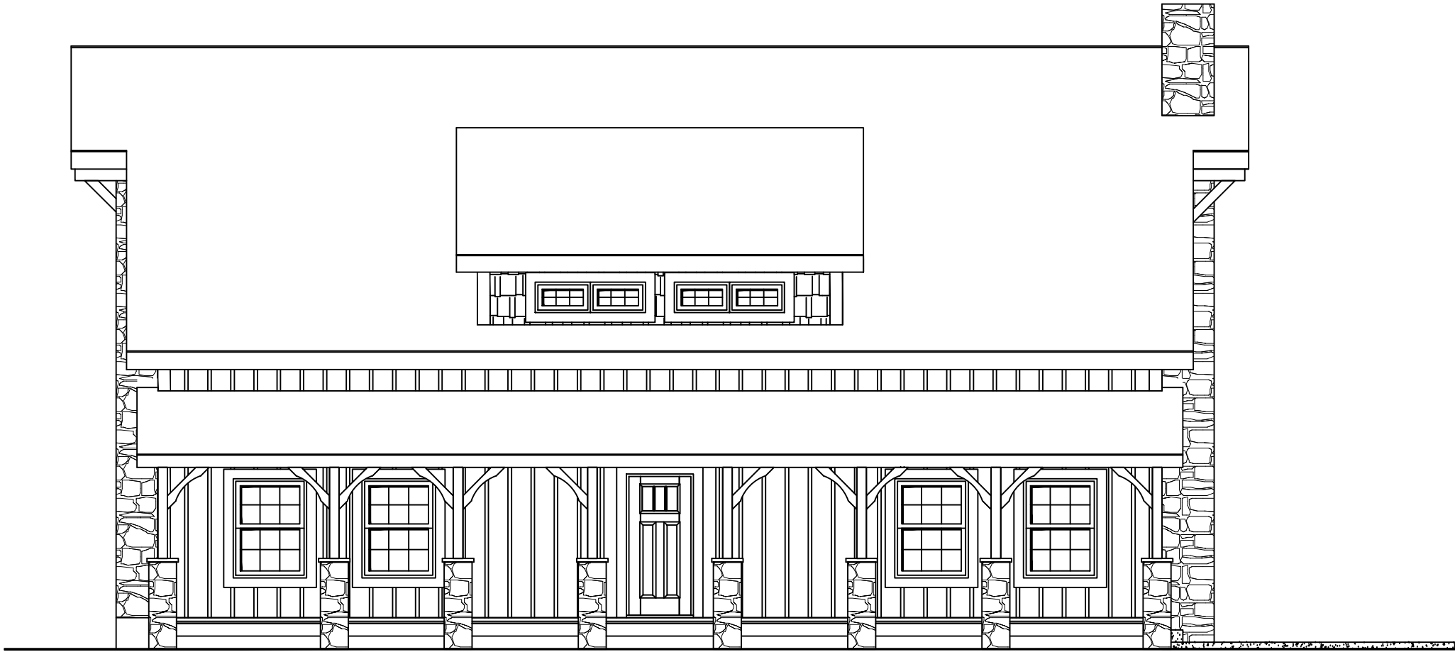
FRONT ELEVATION
