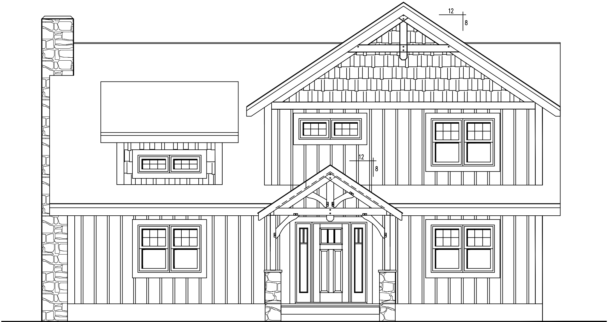
FRONT ELEVATION
