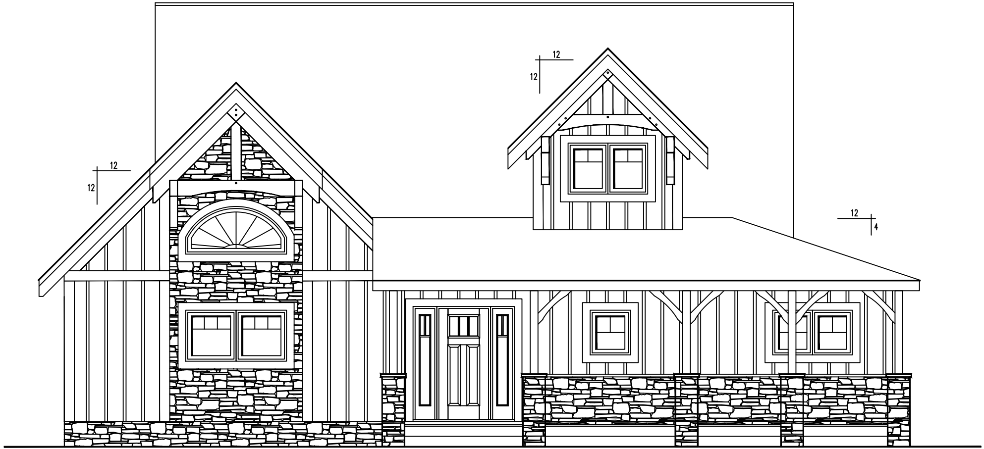
FRONT ELEVATION
