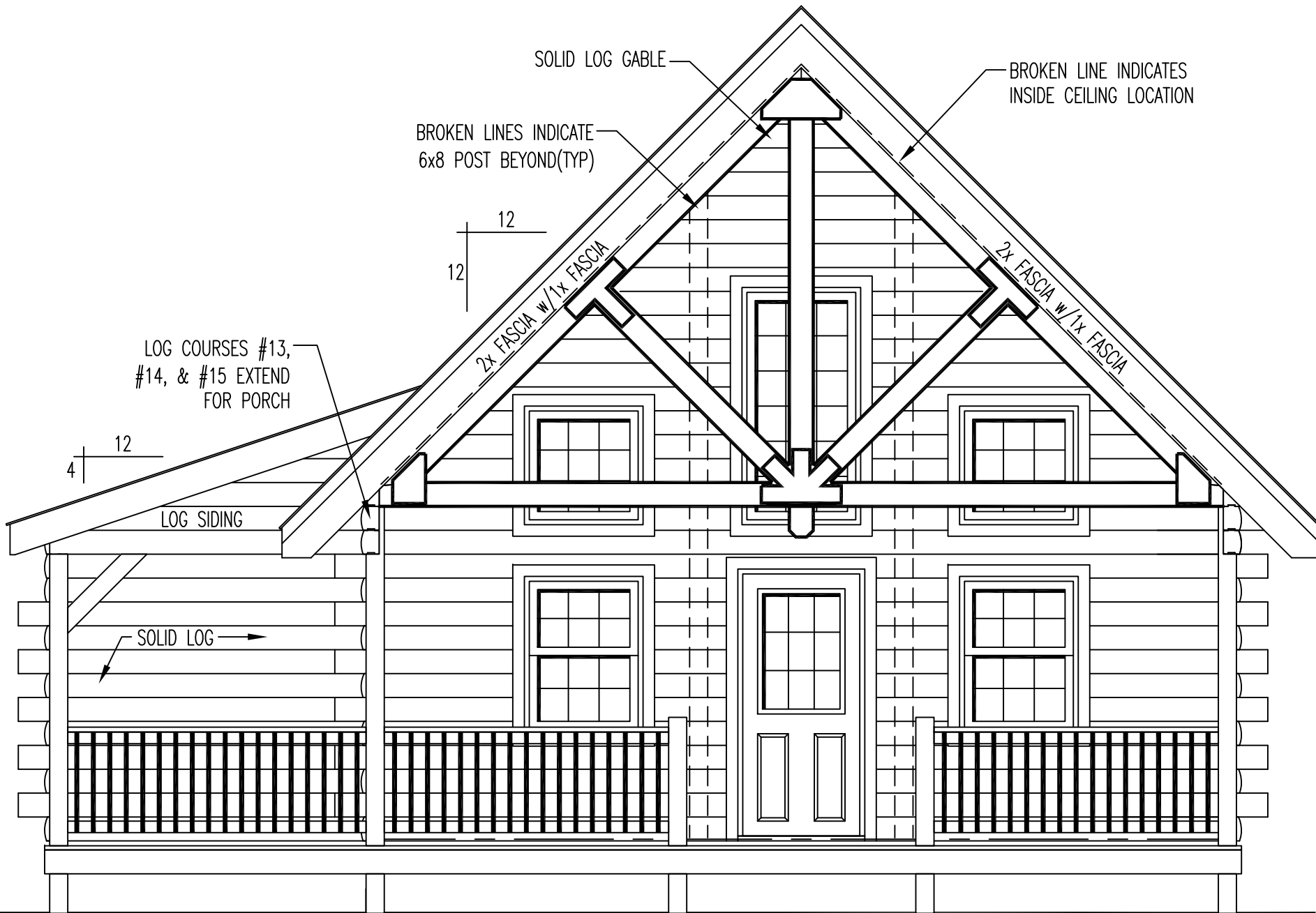
FRONT ELEVATION
