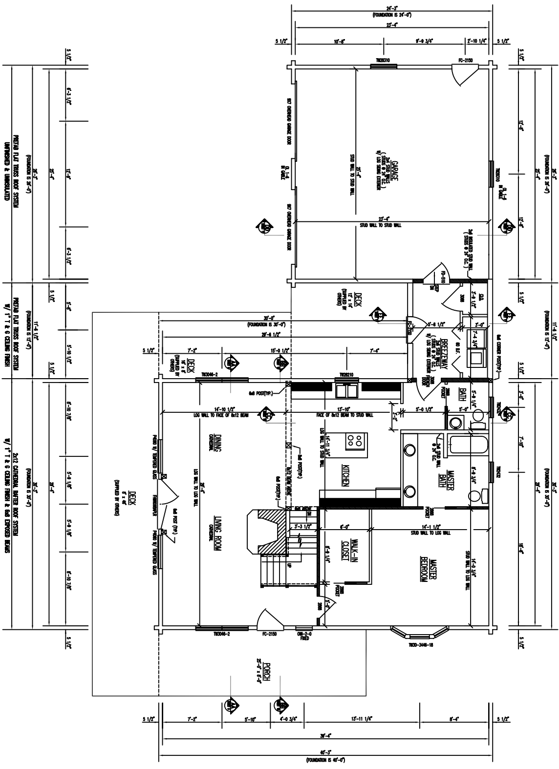
FLOOR PLAN 1st LEVEL
