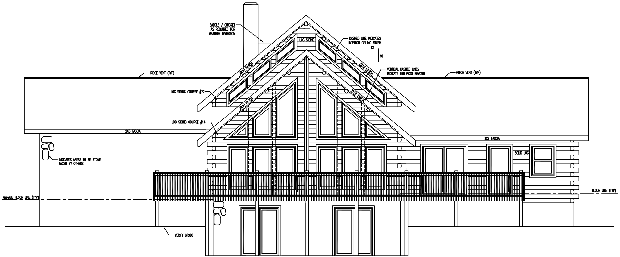
REAR ELEVATION
