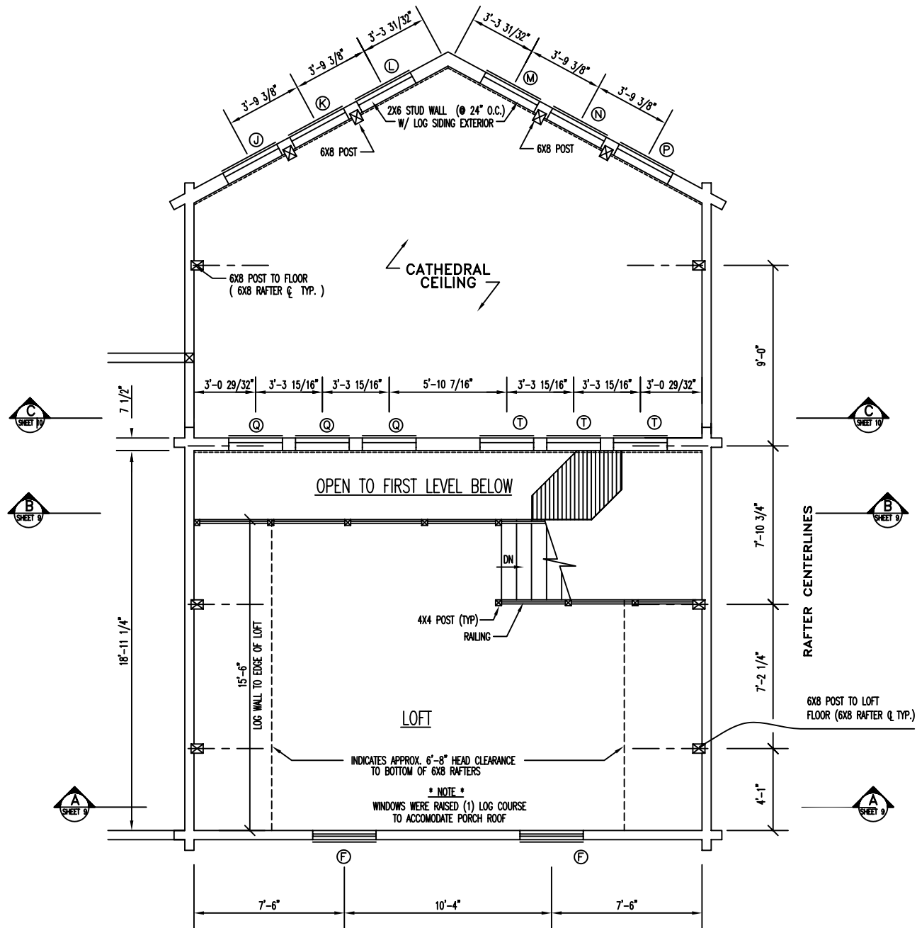
FLOOR PLAN 2nd LEVEL
