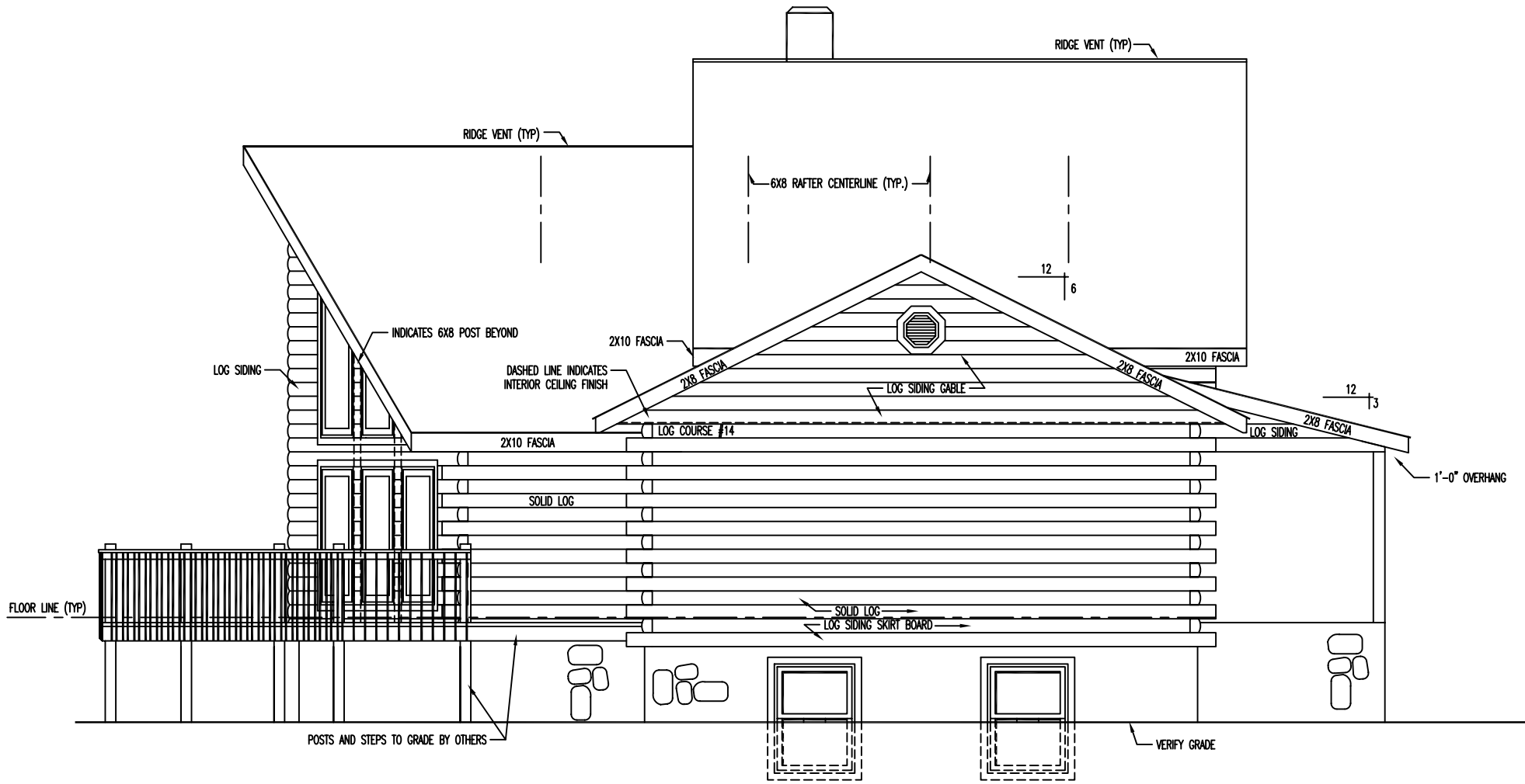
LEFT ELEVATION
