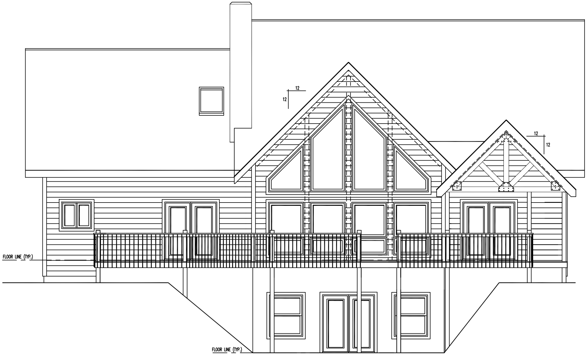
REAR ELEVATION
