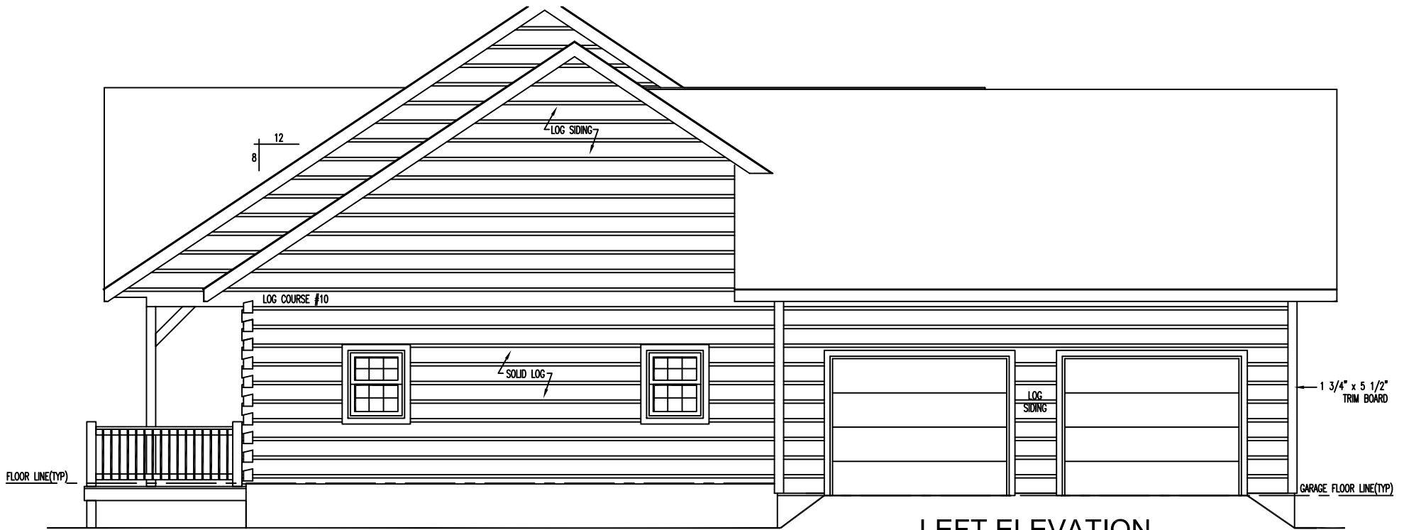
LEFT ELEVATION
