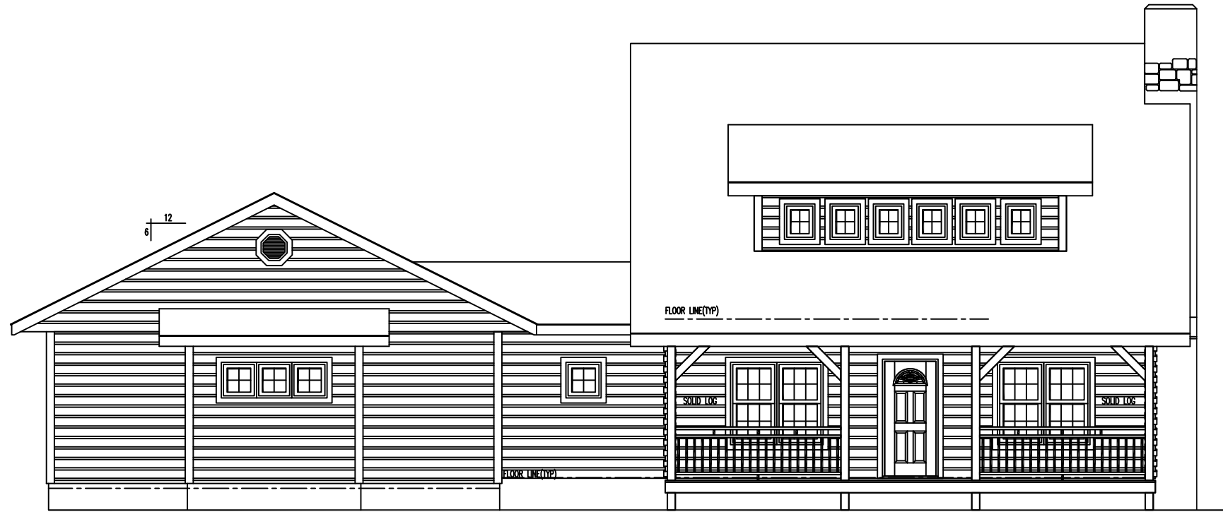
FRONT ELEVATION
