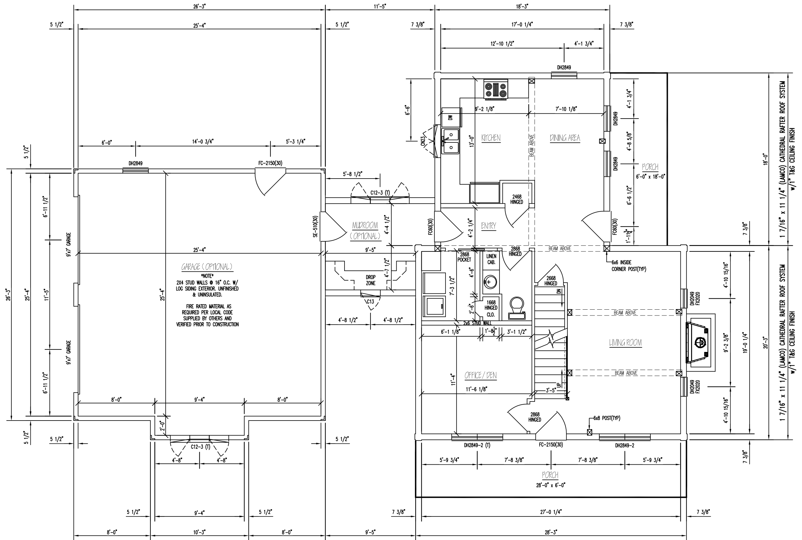
1st LEVEL FLOOR PLAN
