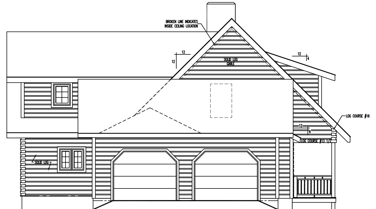
LEFT ELEVATION
