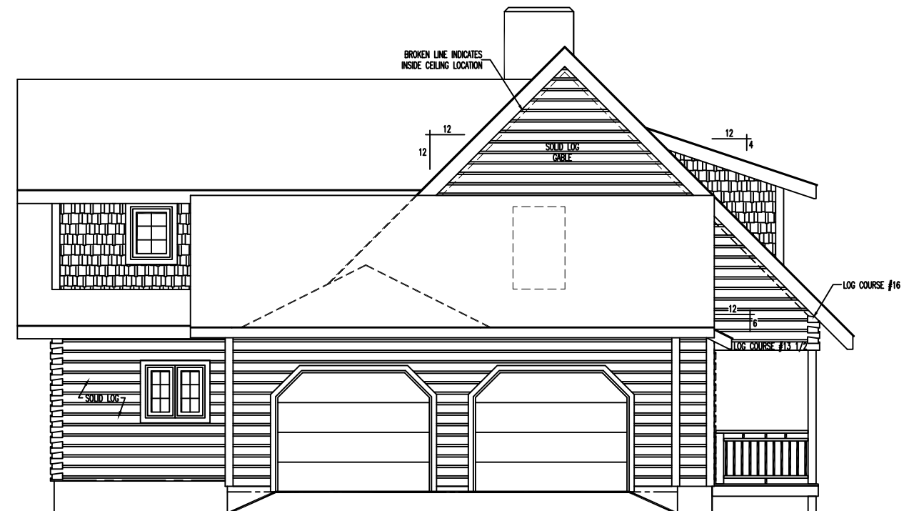
LEFT ELEVATION
