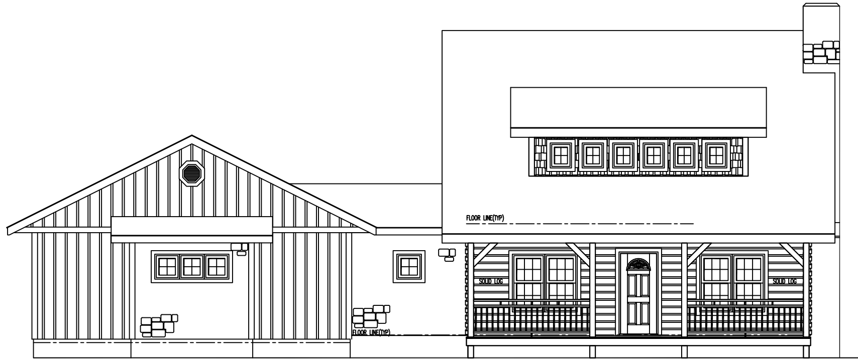
FRONT ELEVATION
