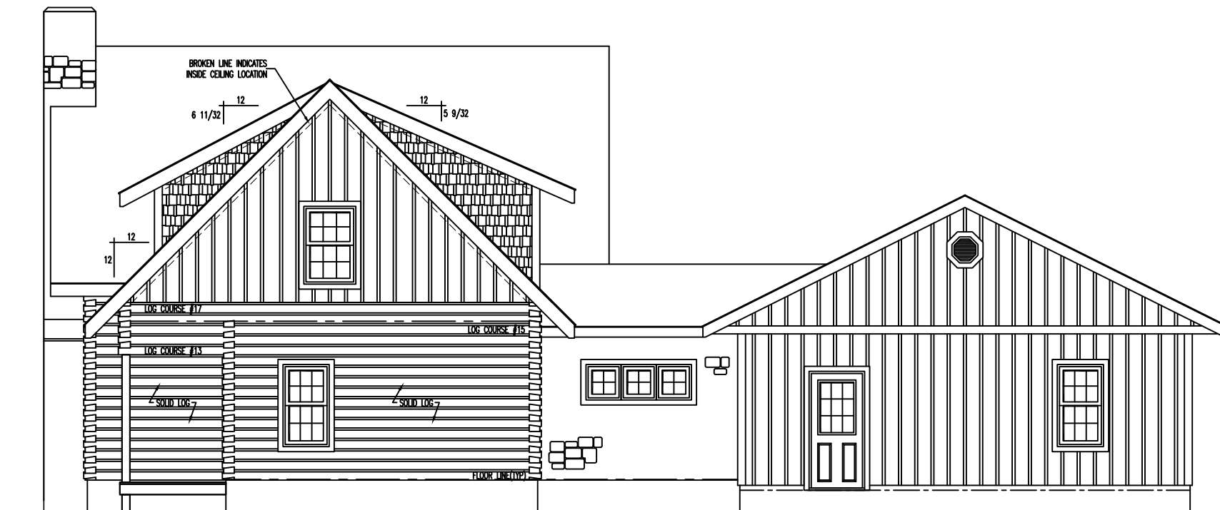
REAR ELEVATION
