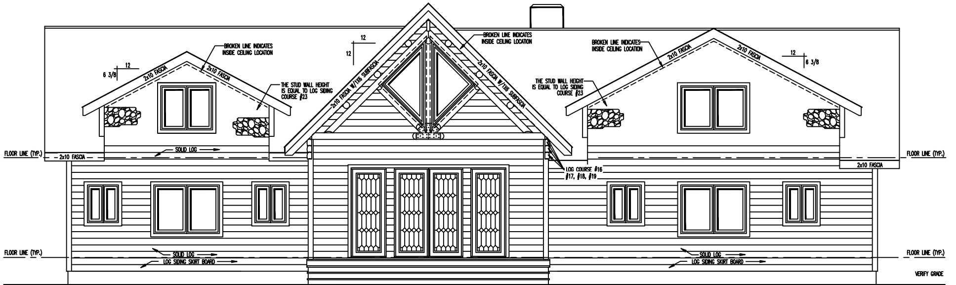
FRONT ELEVATION
