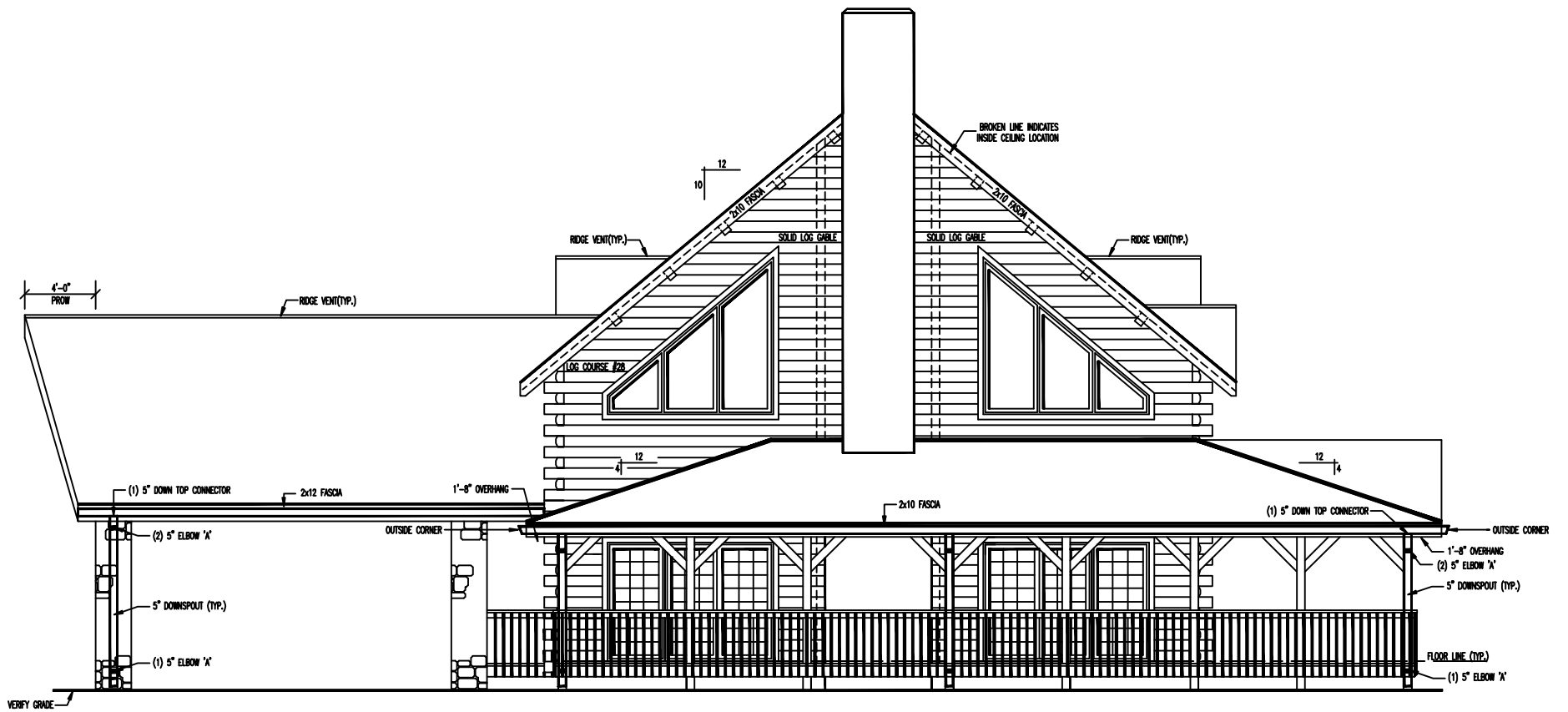
FRONT ELEVATION
