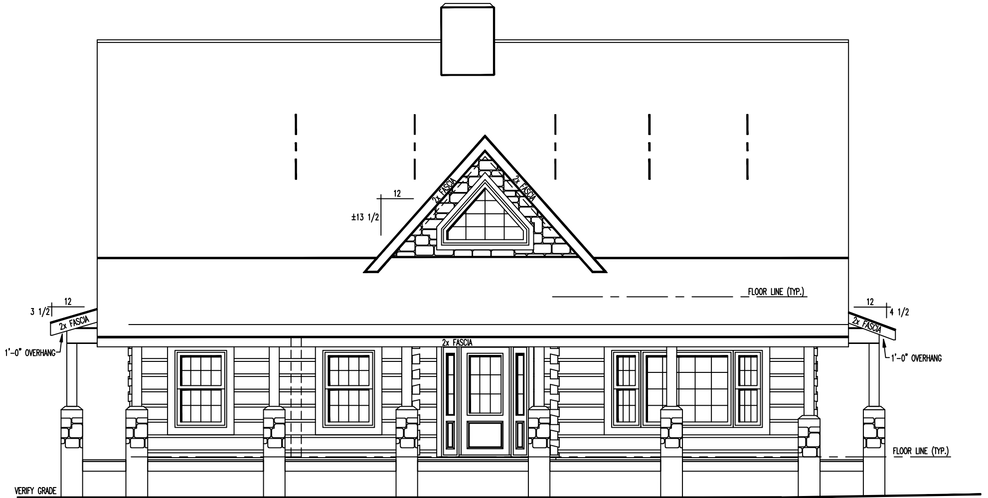
FRONT ELEVATION
