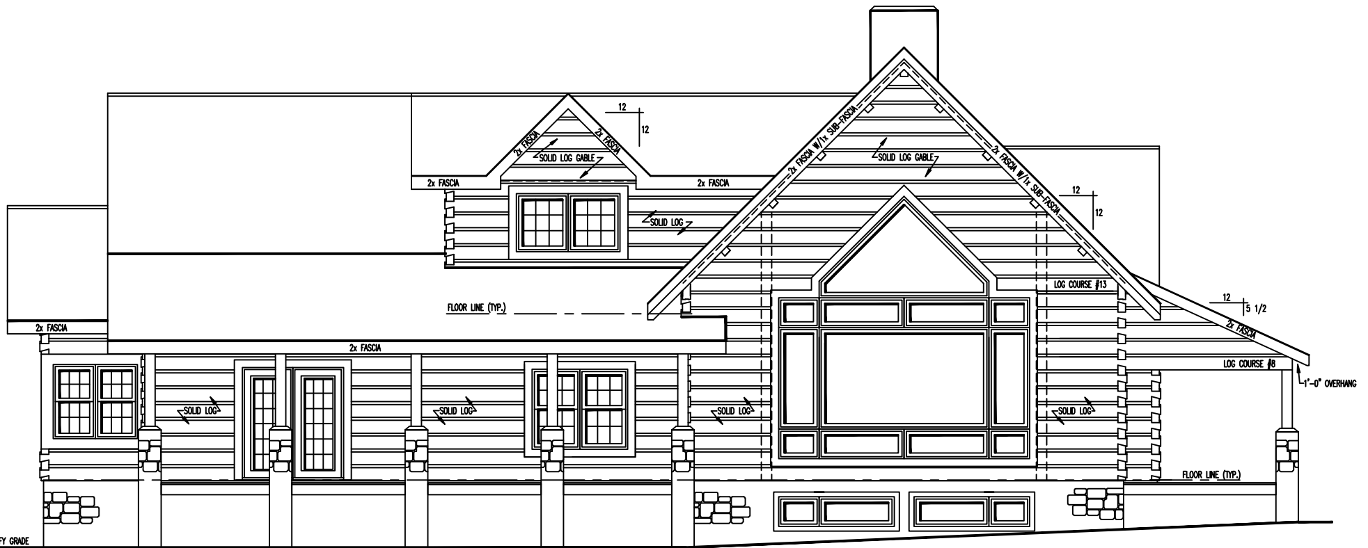
LEFT ELEVATION
