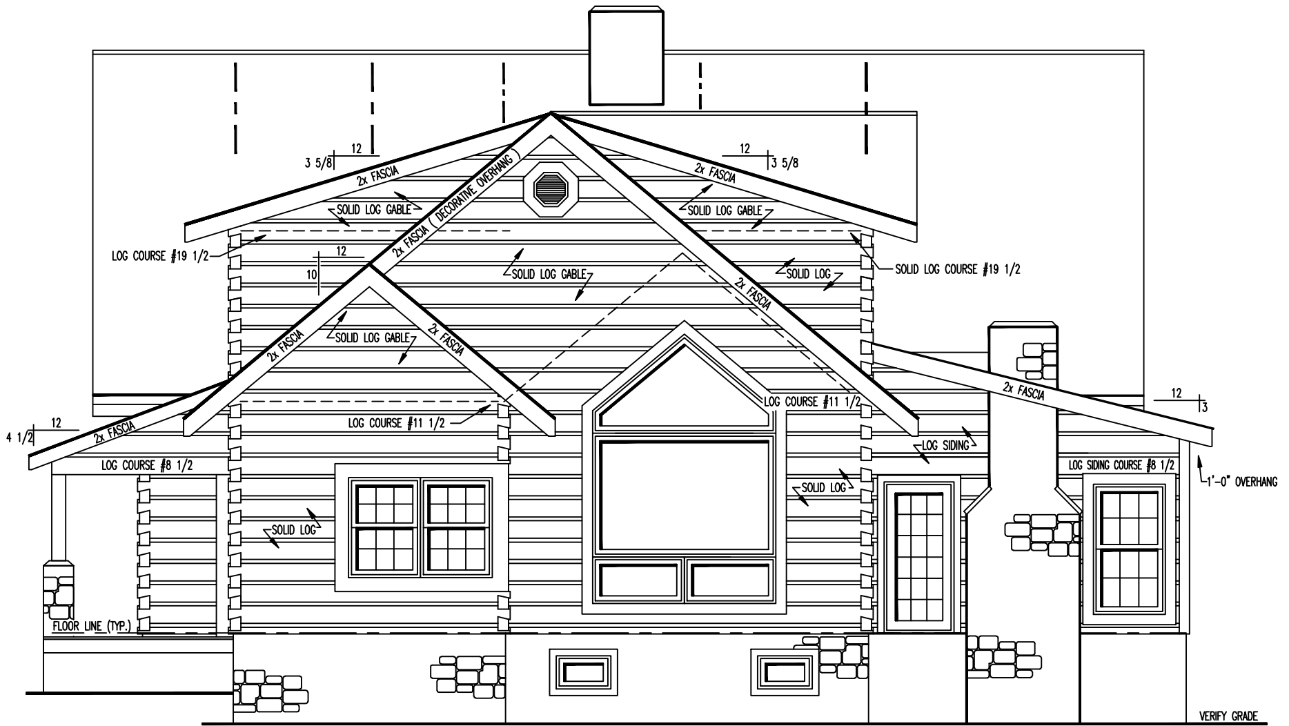
REAR ELEVATION
