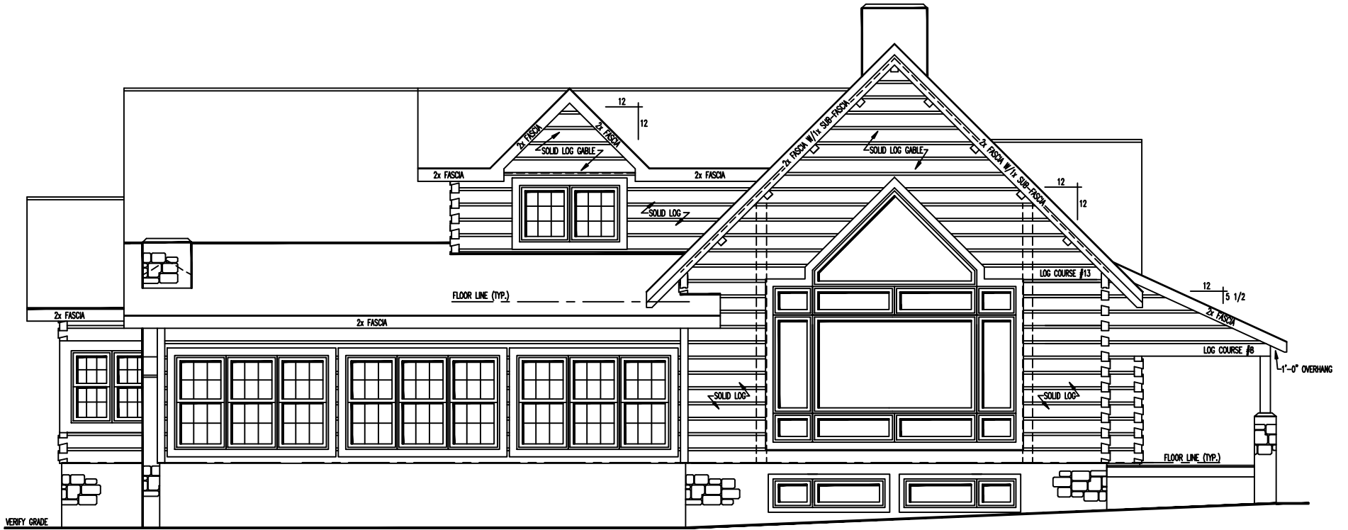
LEFT ELEVATION
