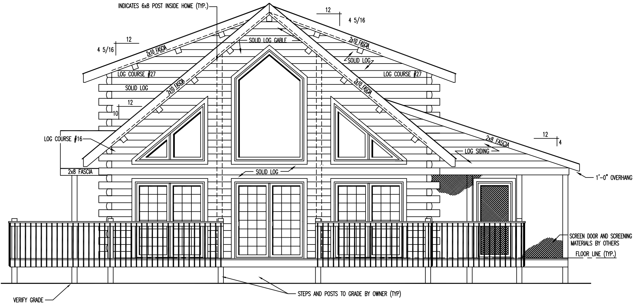
FRONT ELEVATION
