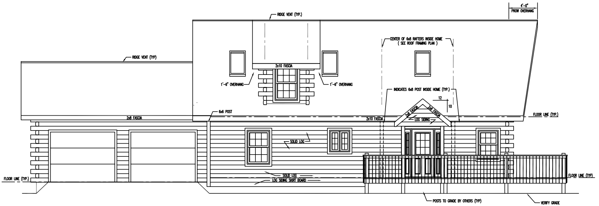
LEFT ELEVATION
