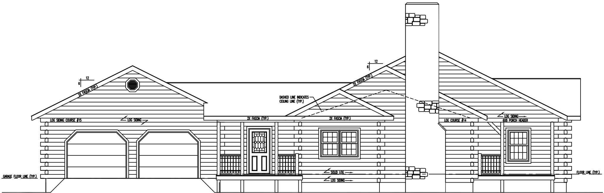
LEFT ELEVATION
