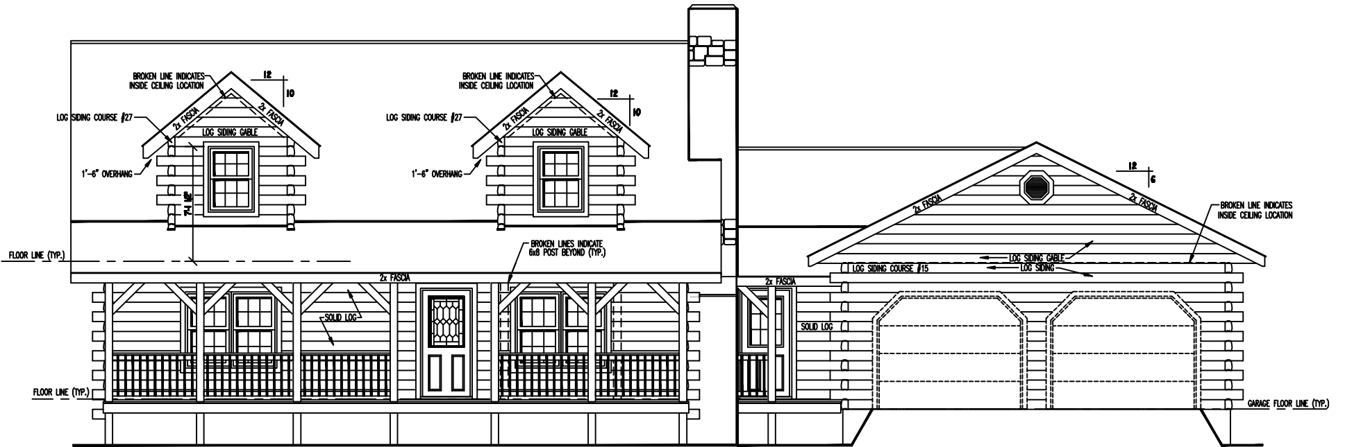
FRONT ELEVATION
