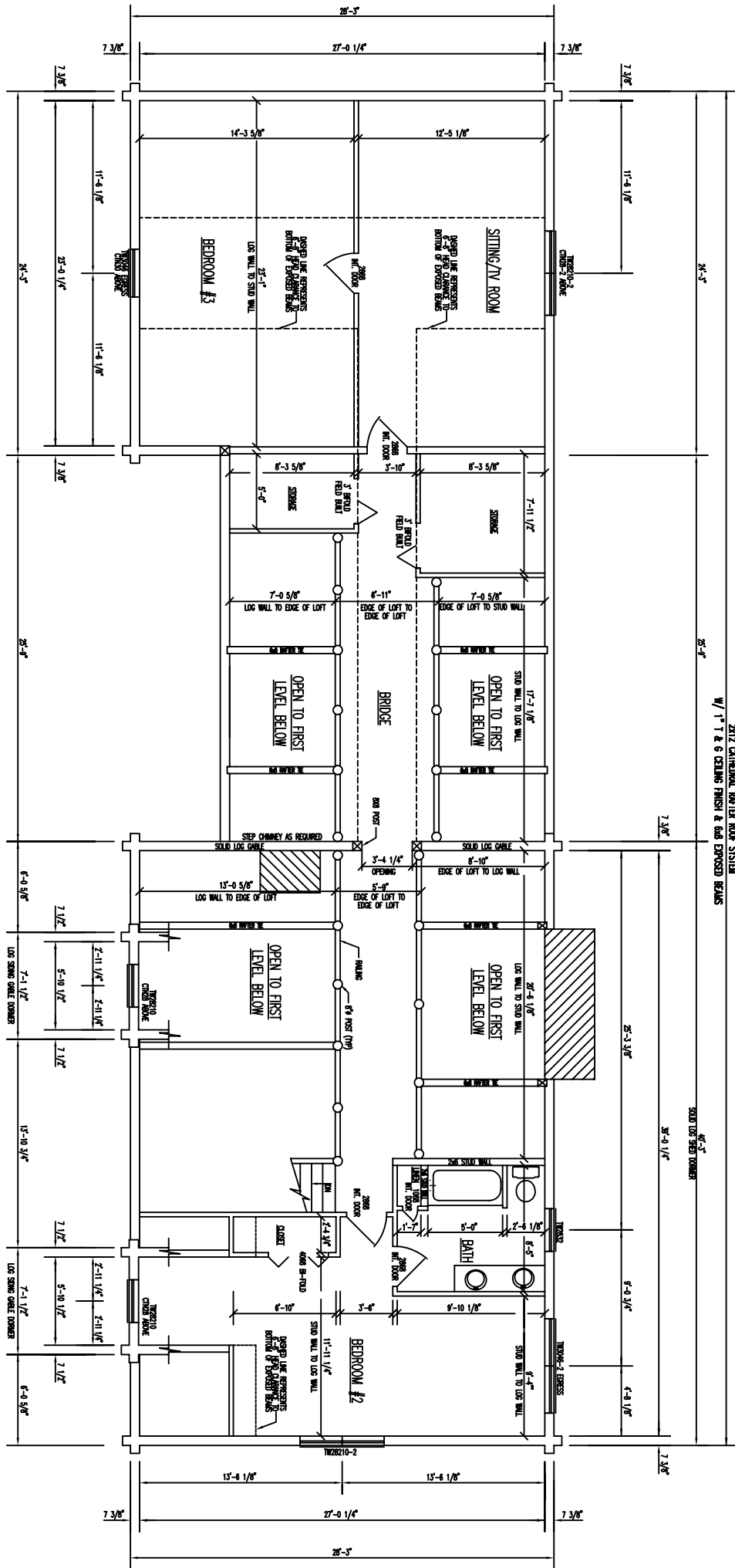
FLOOR PLAN 2ND LEVEL FLOOR AREA = 1516 SQ. FT. HOUSE
