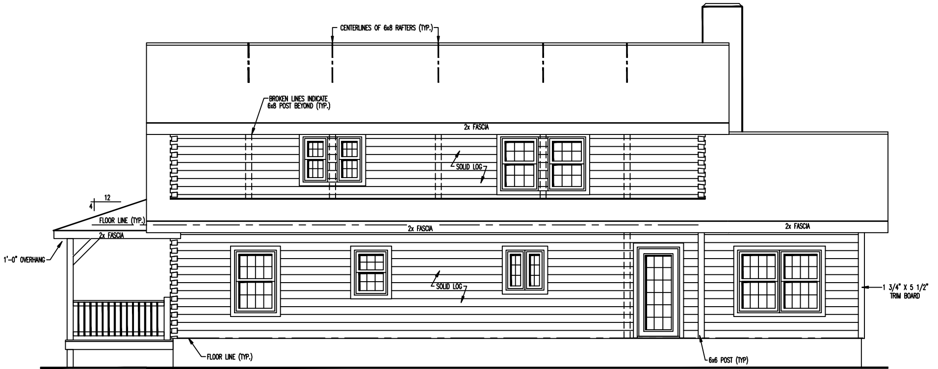
REAR ELEVATION
