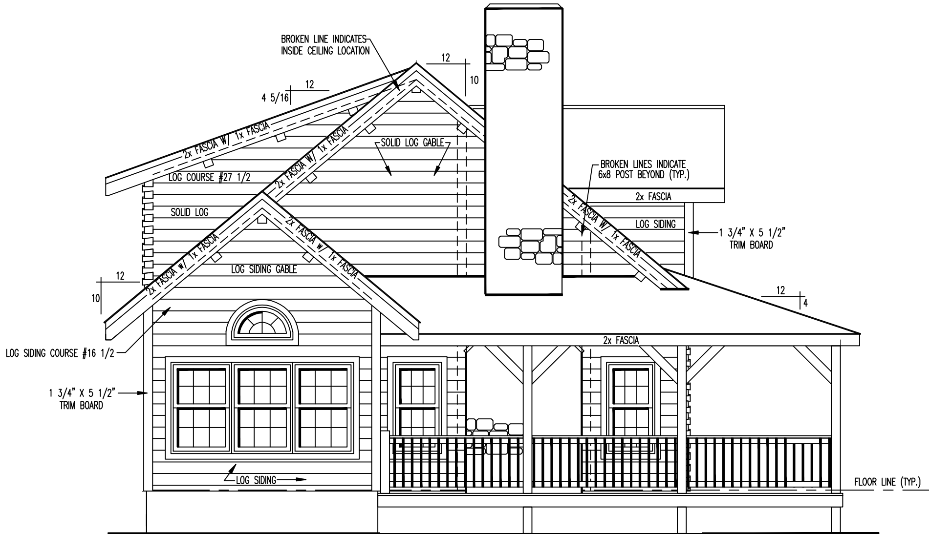
LEFT ELEVATION
