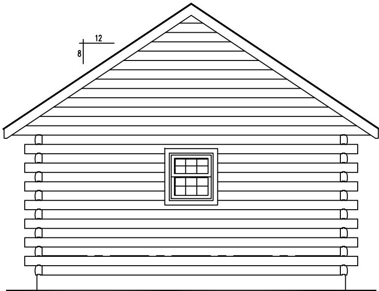
REAR ELEVATION
