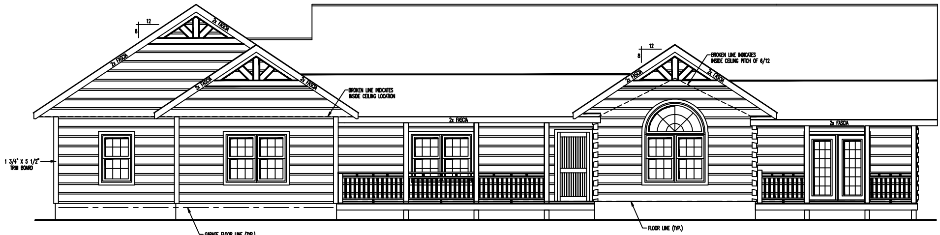
FRONT ELEVATION
