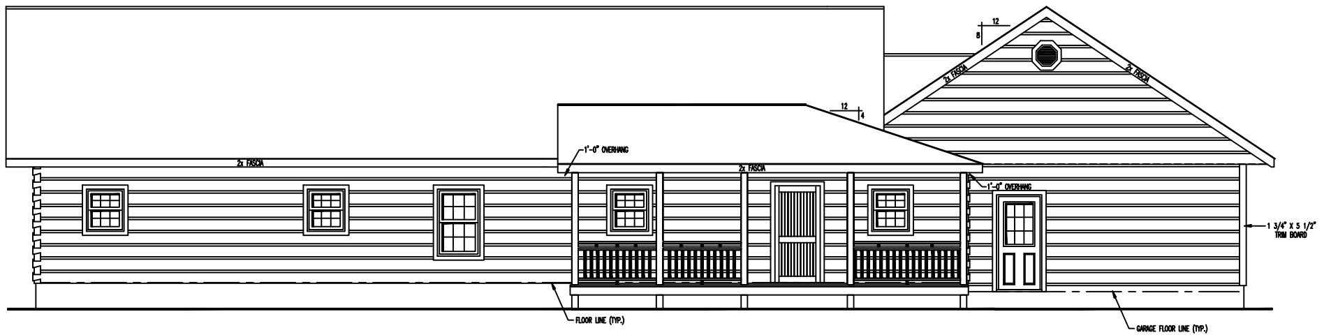
REAR ELEVATION
