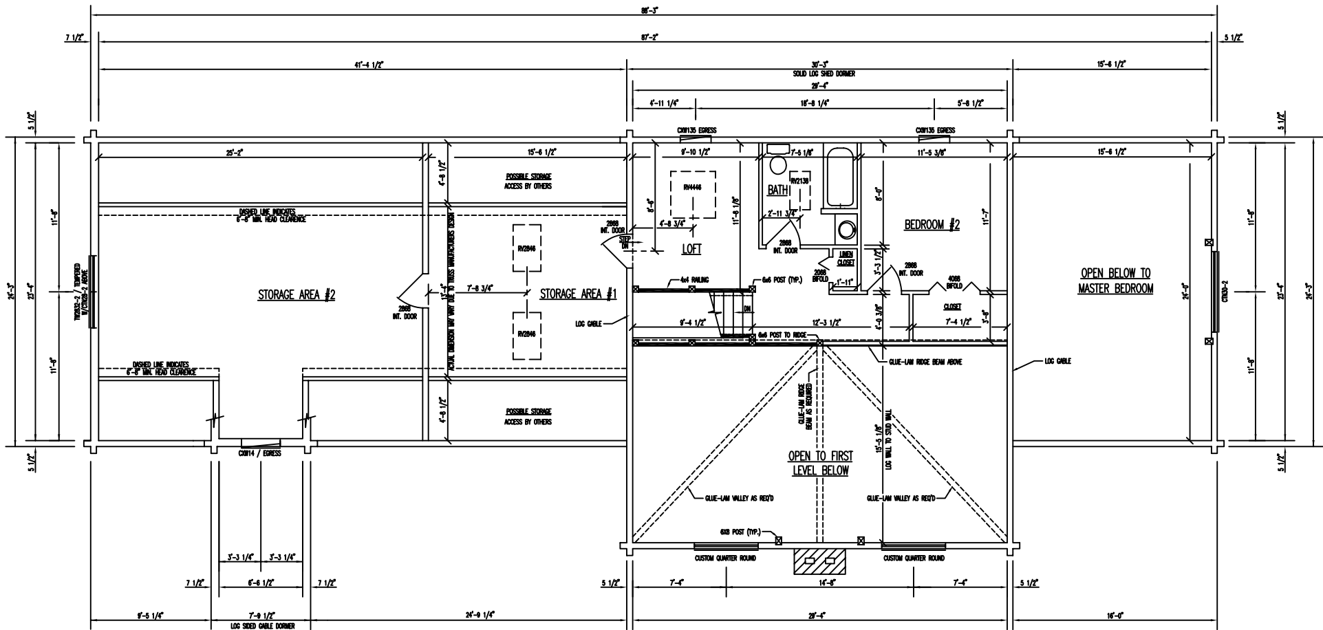
FLOOR PLAN 2nd LEVEL
