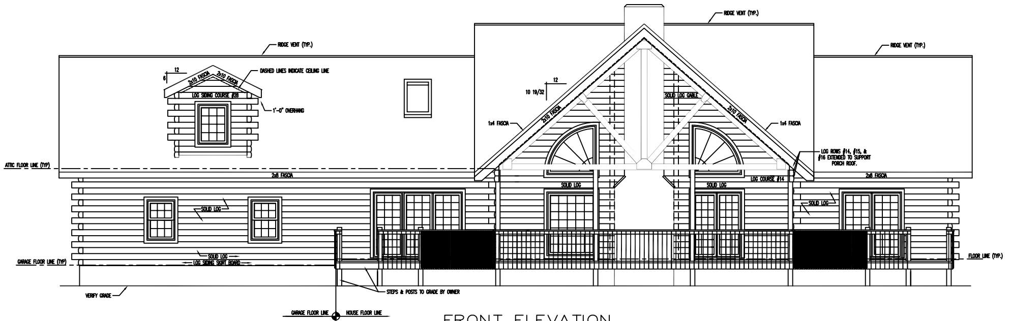
FRONT ELEVATION
