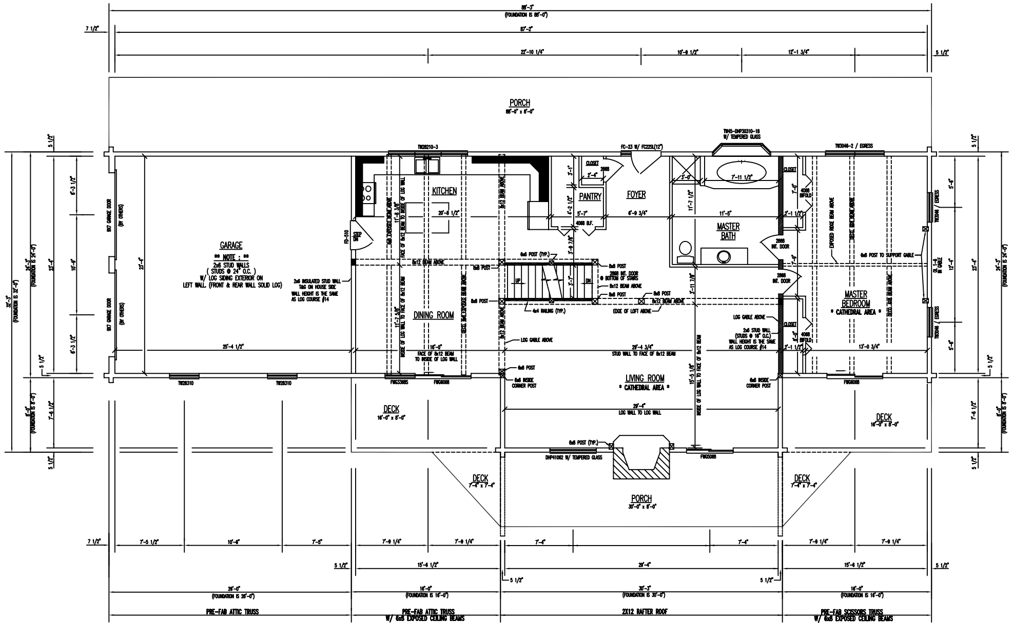
FLOOR PLAN 1st LEVEL
