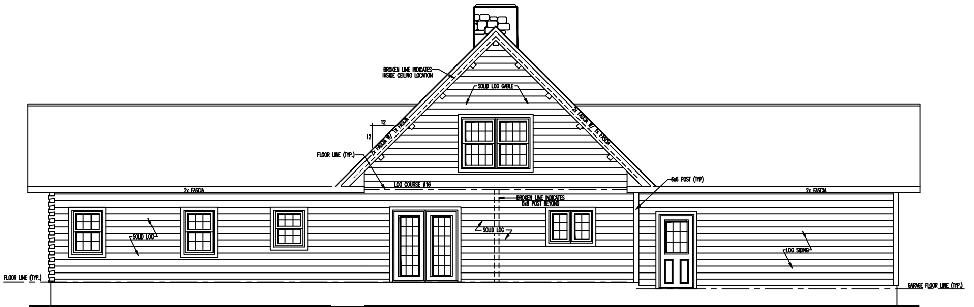
REAR ELEVATION
