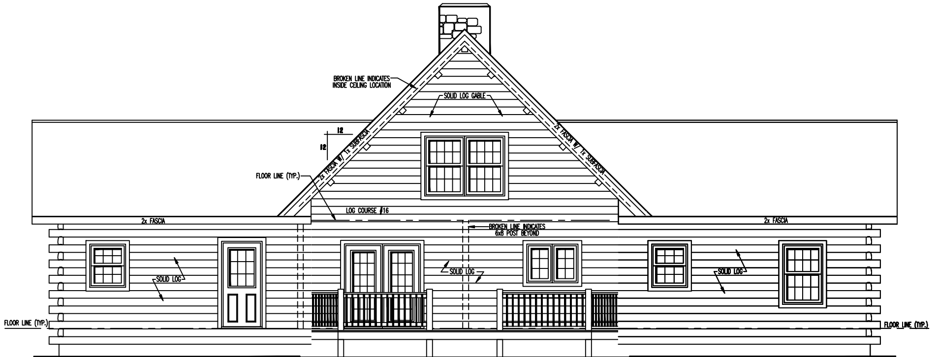
REAR ELEVATION
