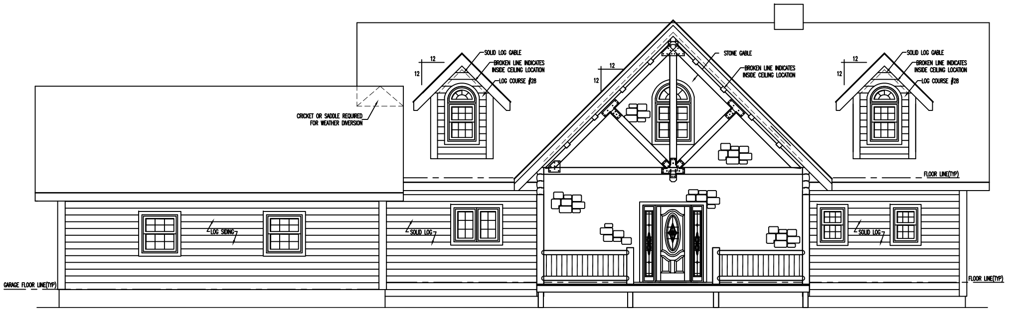
FRONT ELEVATION
