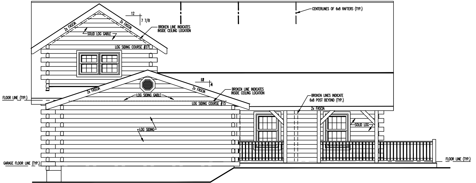
FRONT ELEVATION
