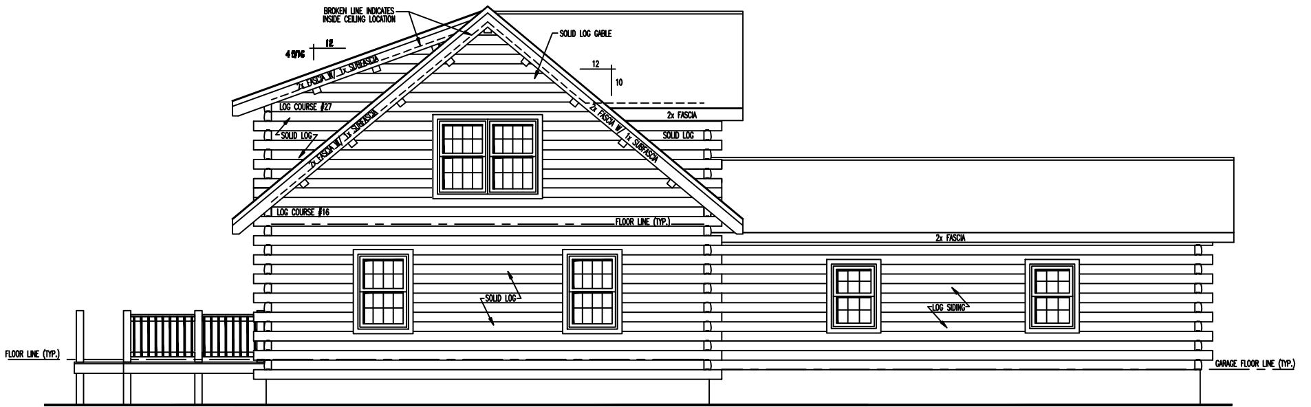
LEFT ELEVATION
