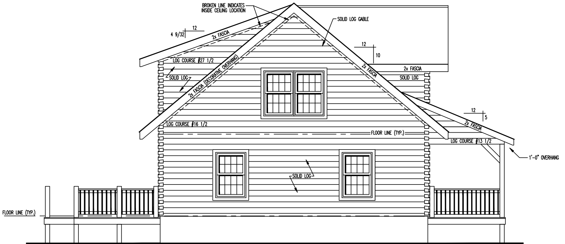
LEFT ELEVATION
