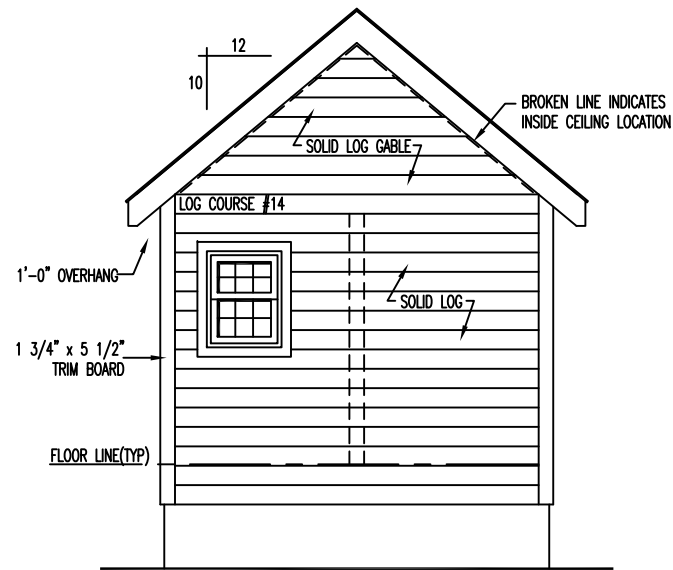
REAR ELEVATION
