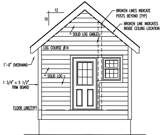
FRONT ELEVATION
