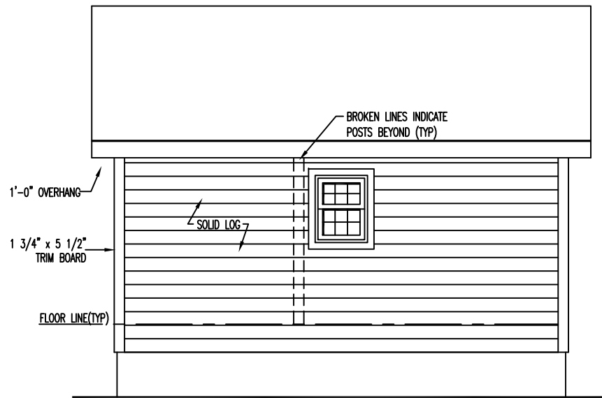
LEFT ELEVATION
