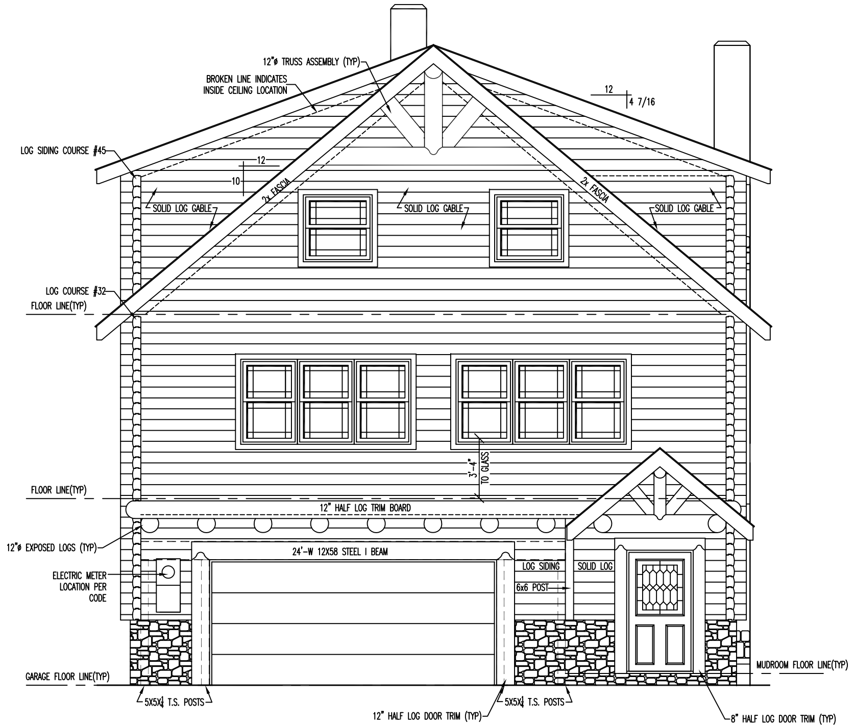
FRONT ELEVATION
