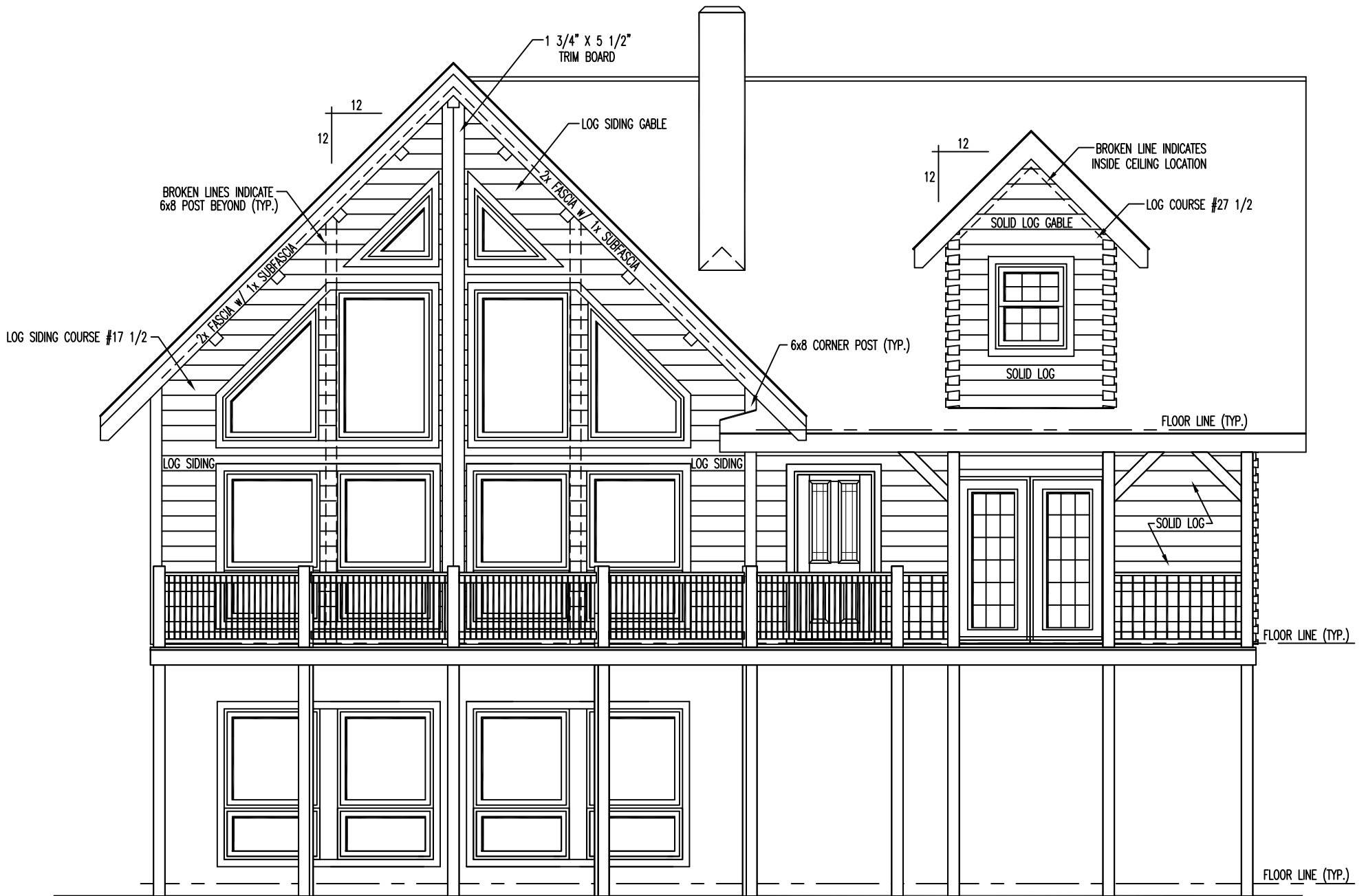
FRONT ELEVATION
