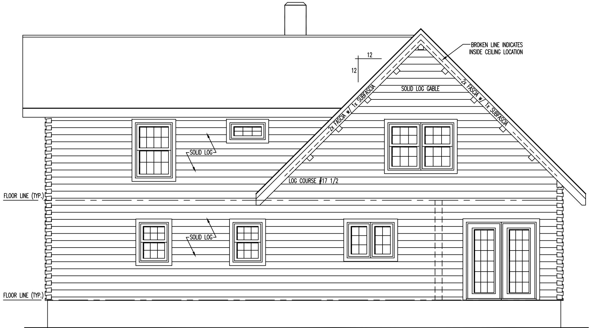
REAR ELEVATION
