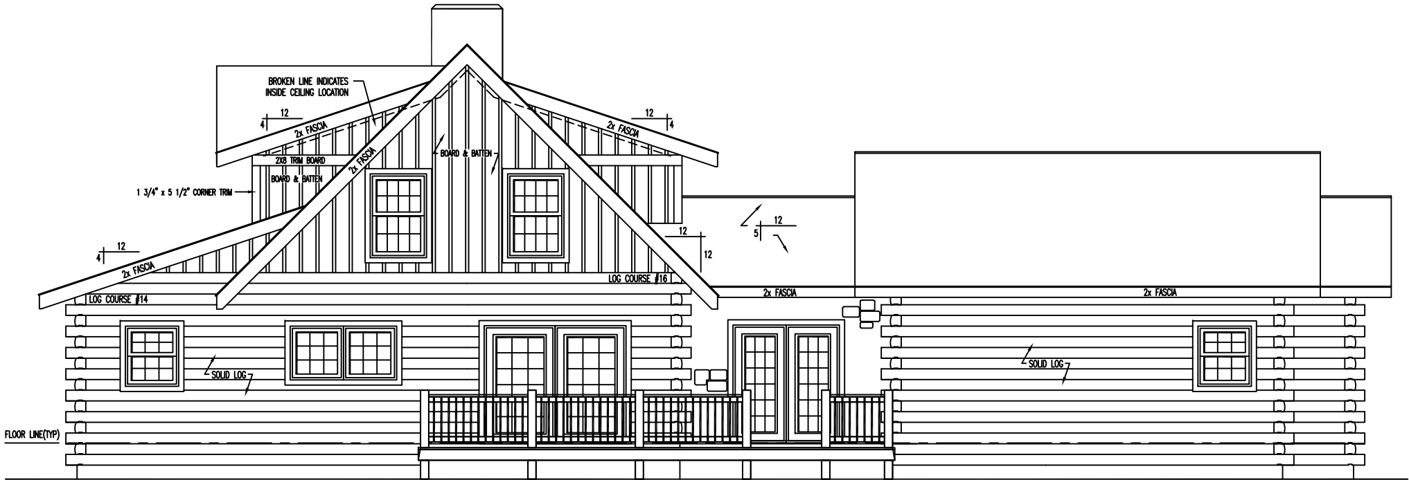
REAR ELEVATION
