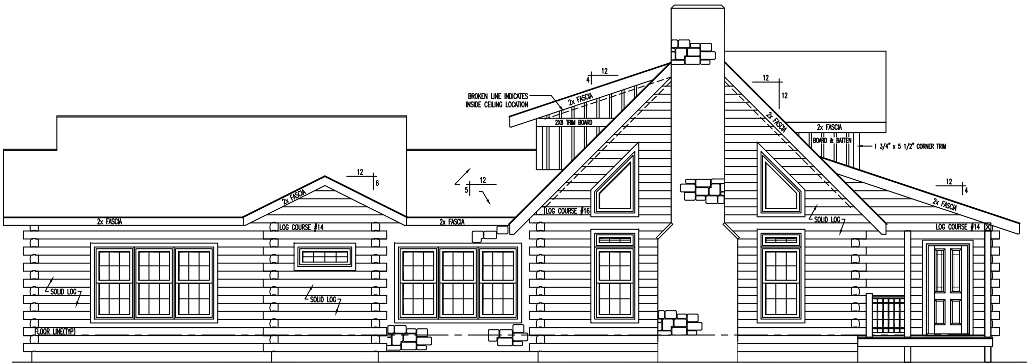
FRONT ELEVATION
