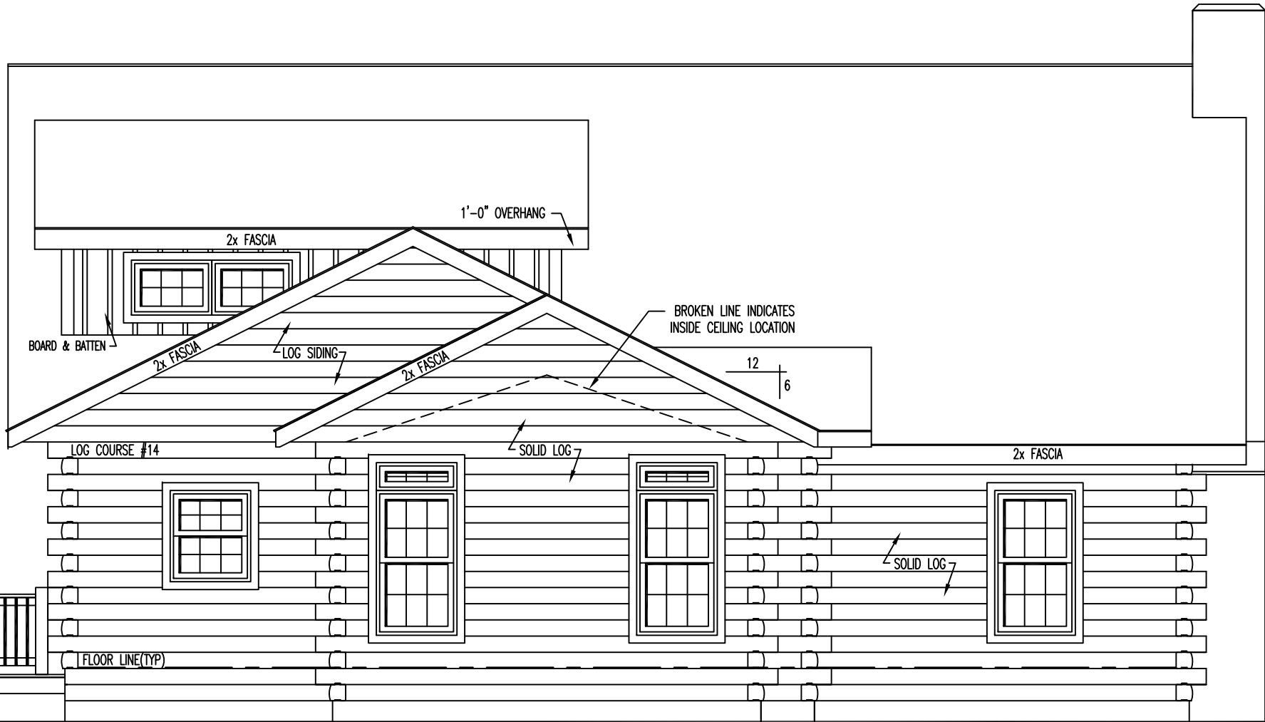
LEFT ELEVATION
