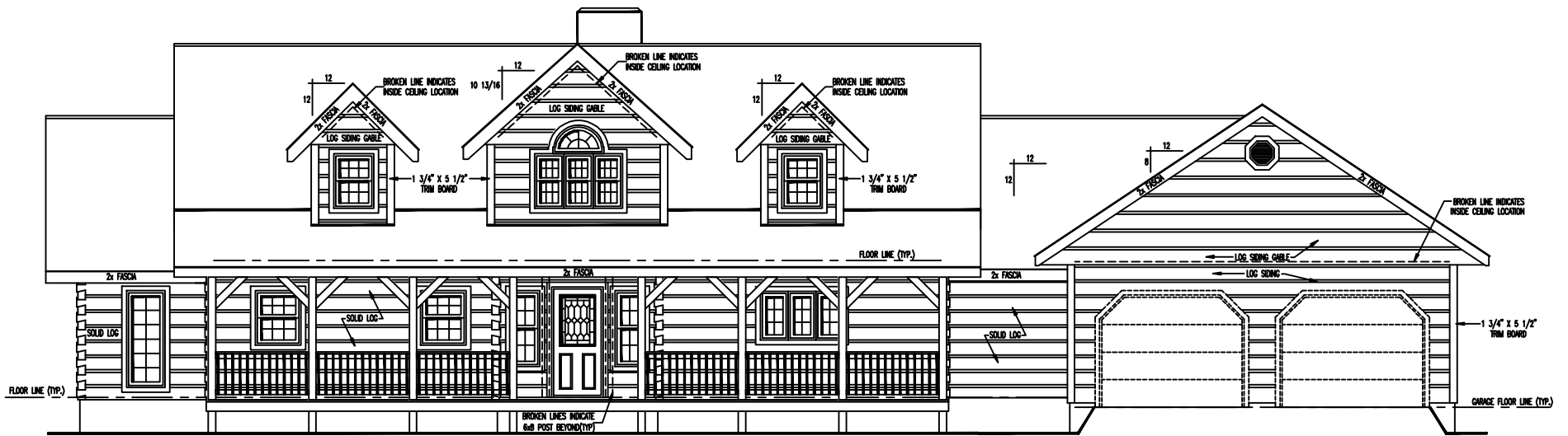
FRONT ELEVATION
