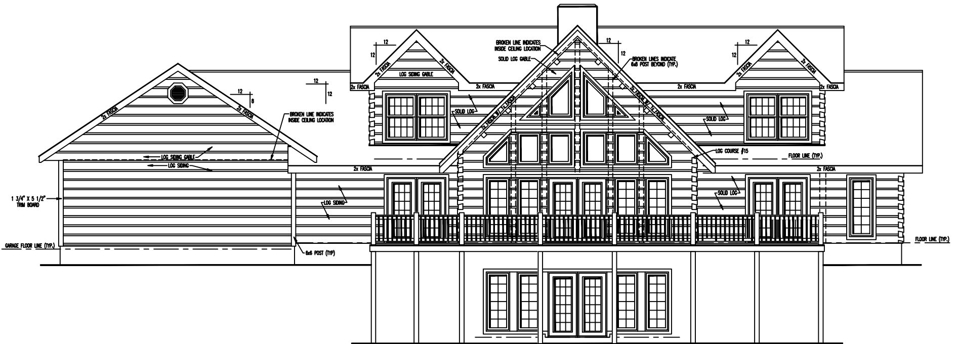
REAR ELEVATION
