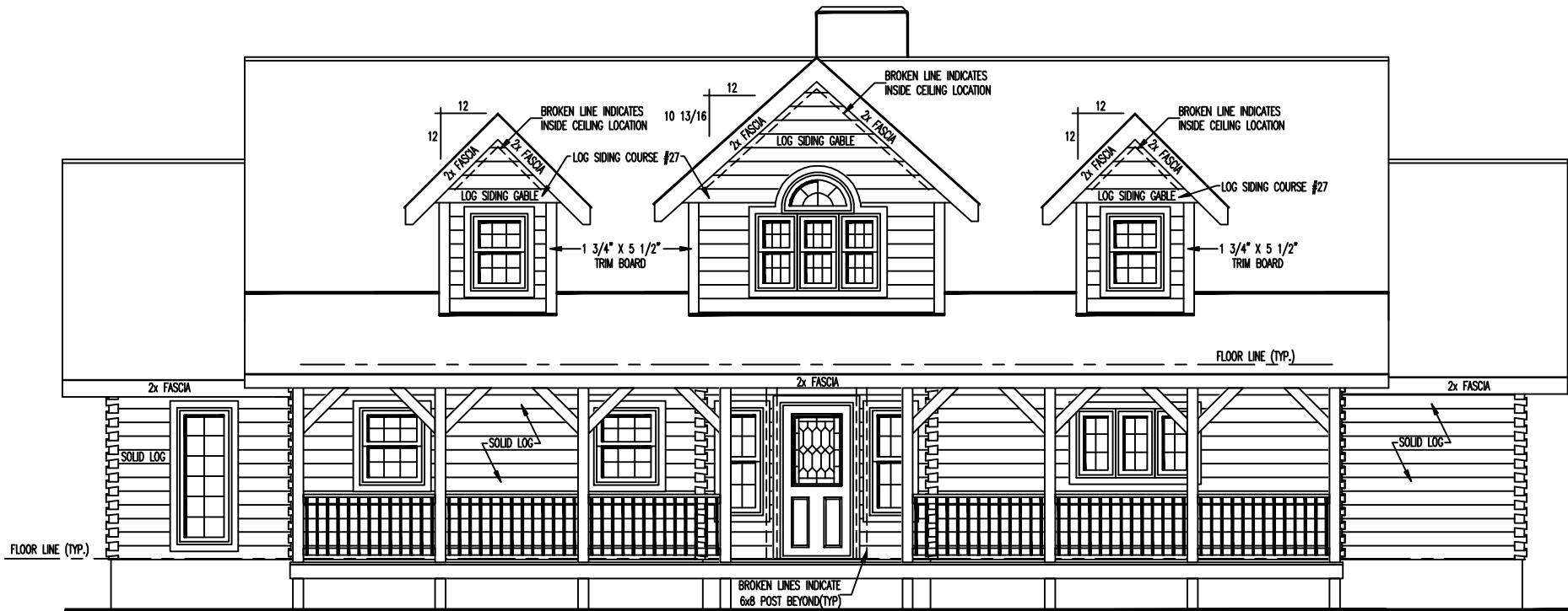
FRONT ELEVATION
