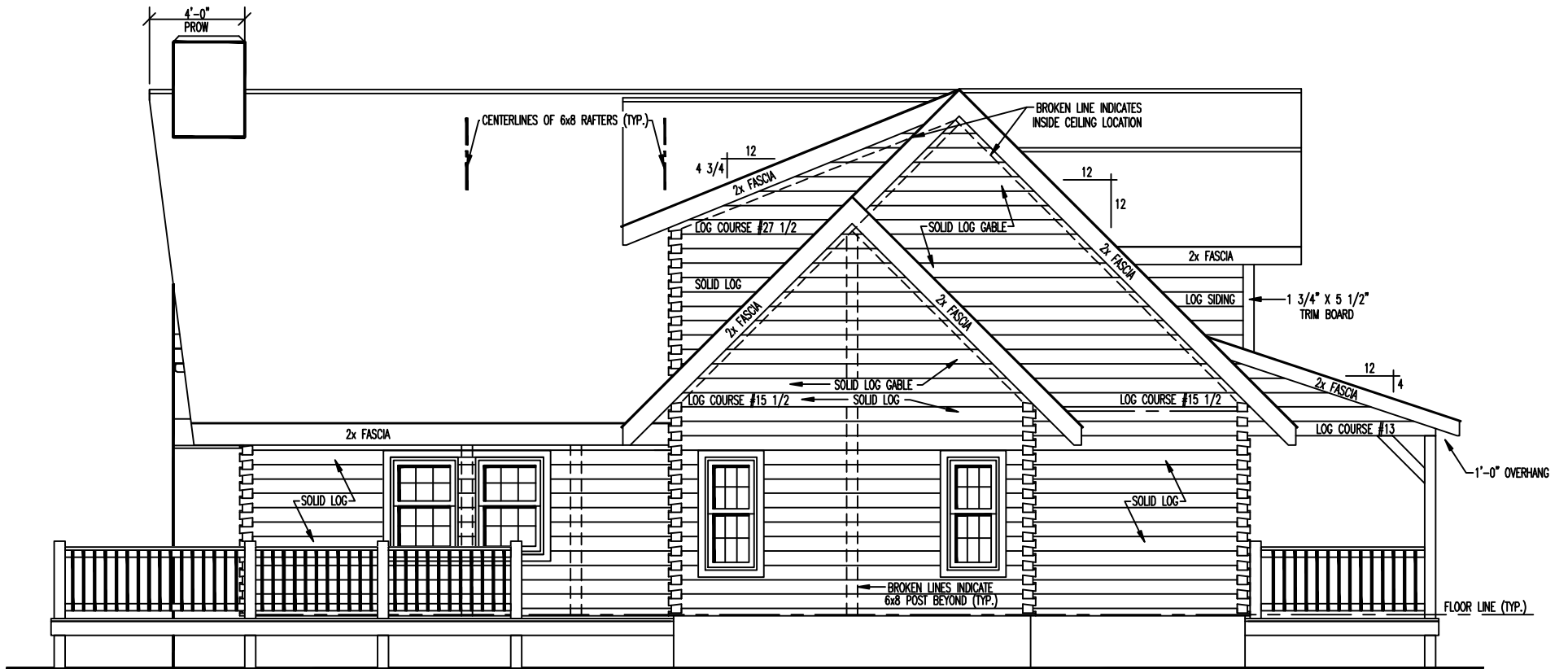
LEFT ELEVATION
