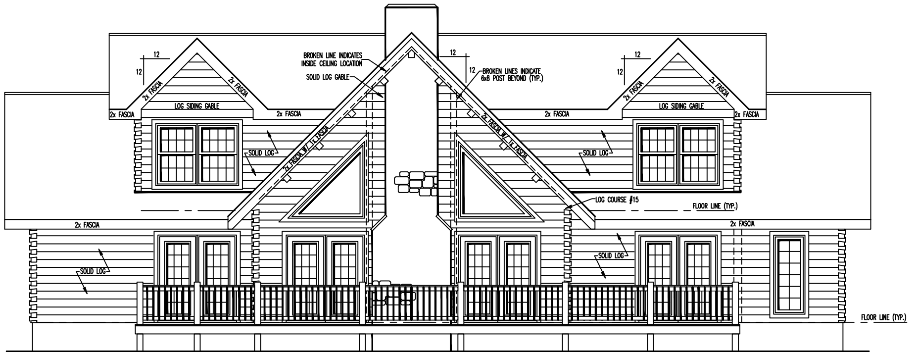
REAR ELEVATION
