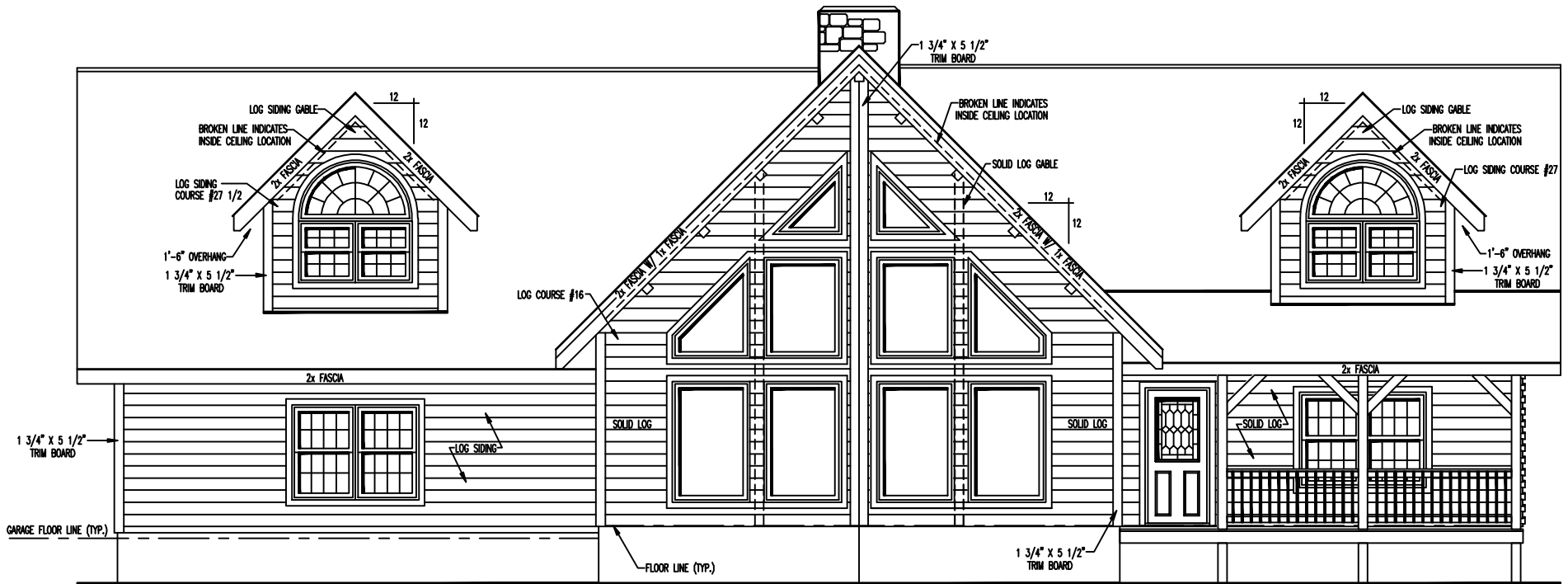
FRONT ELEVATION
