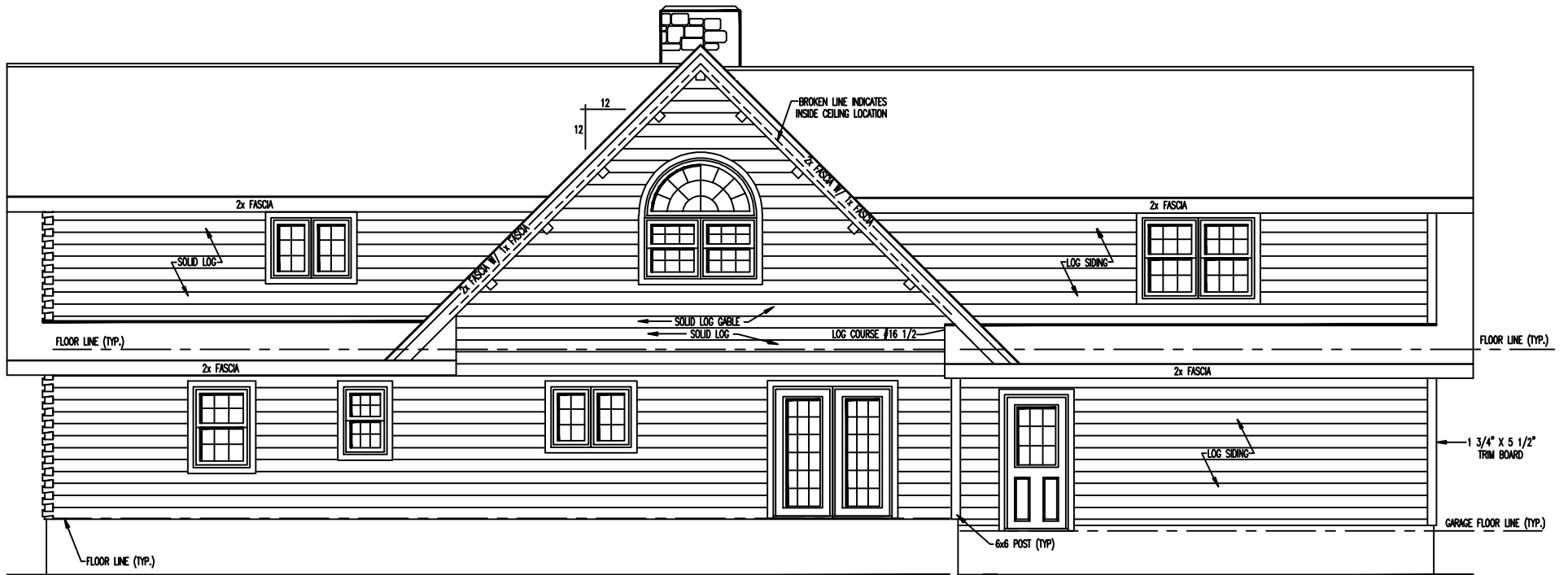
REAR ELEVATION
