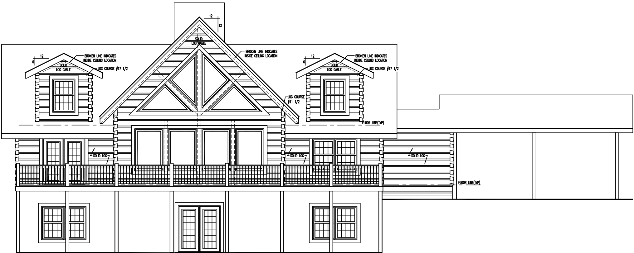
REAR ELEVATION
