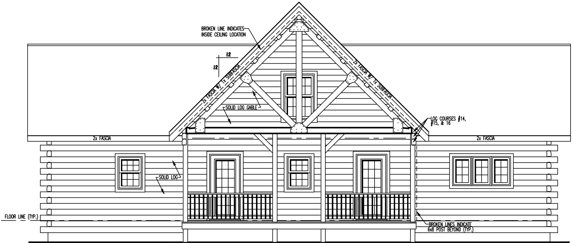
REAR ELEVATION
