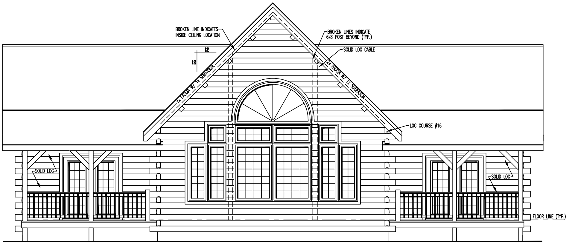
FRONT ELEVATION
