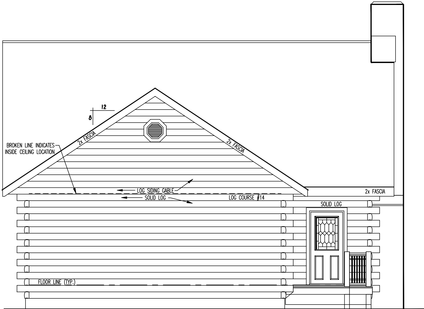
LEFT ELEVATION
