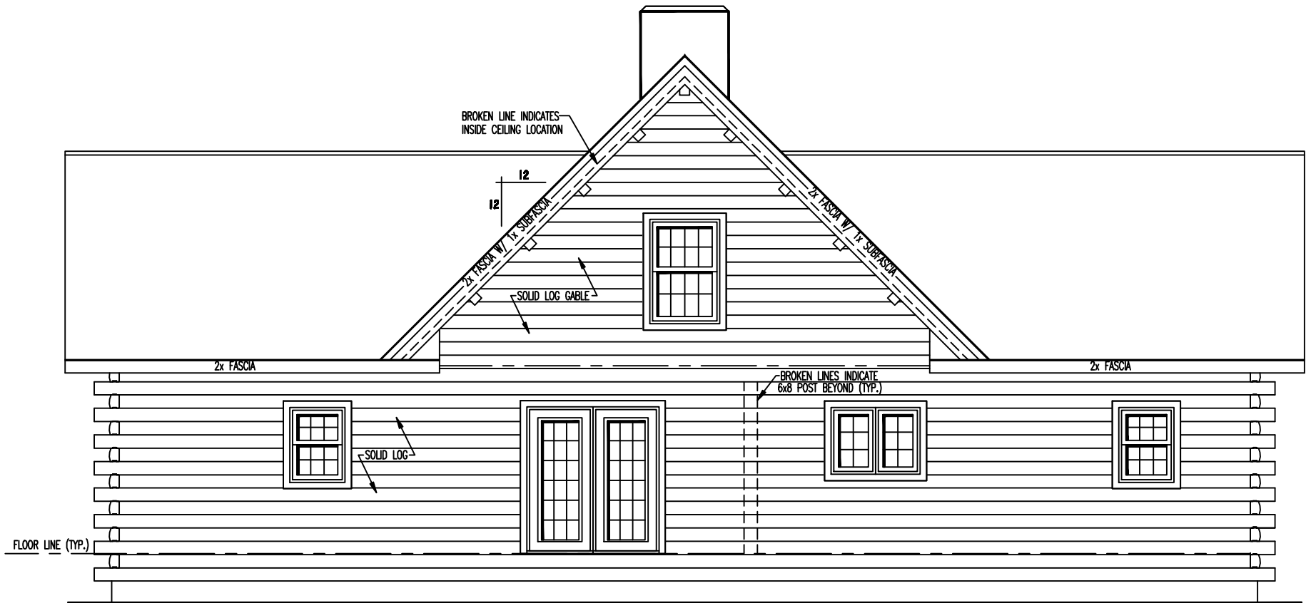
REAR ELEVATION
