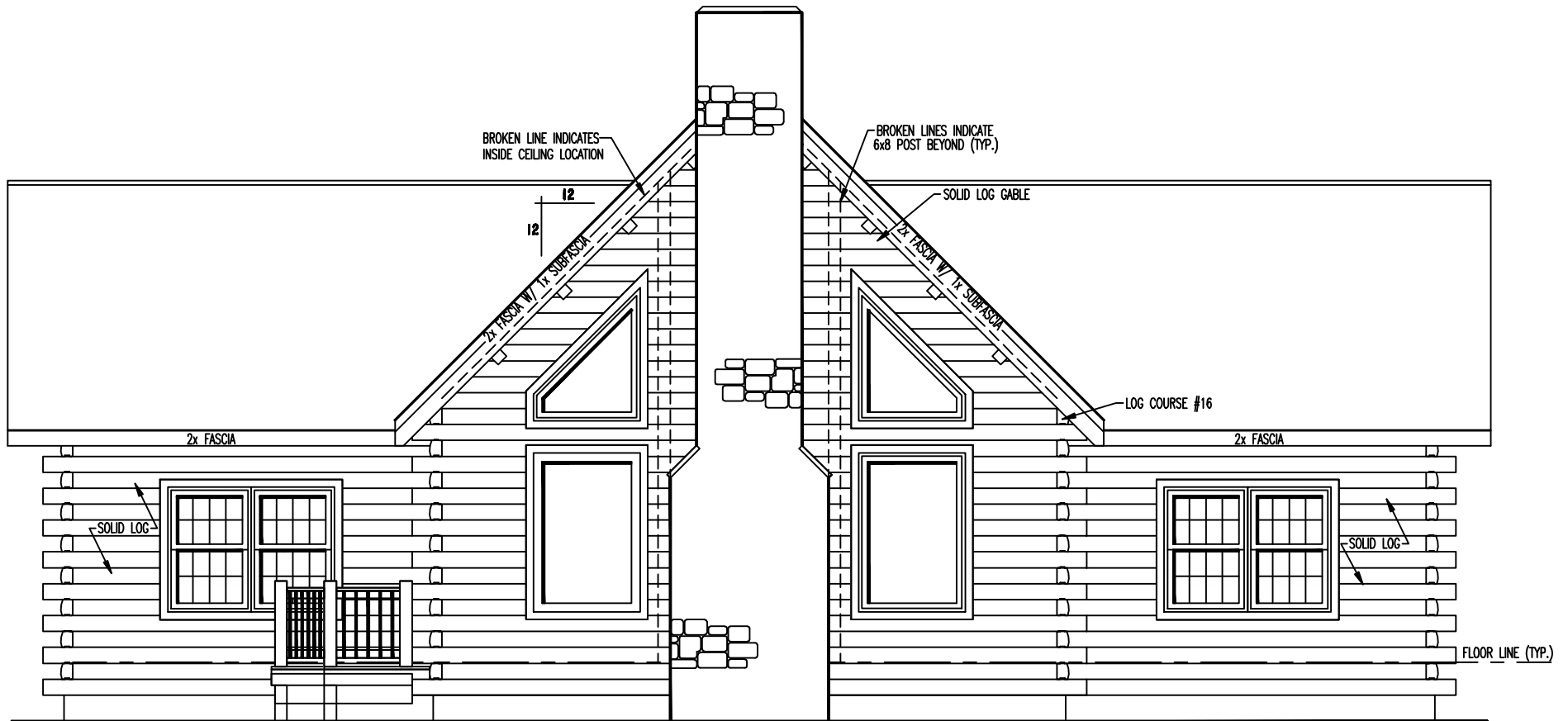
FRONT ELEVATION
