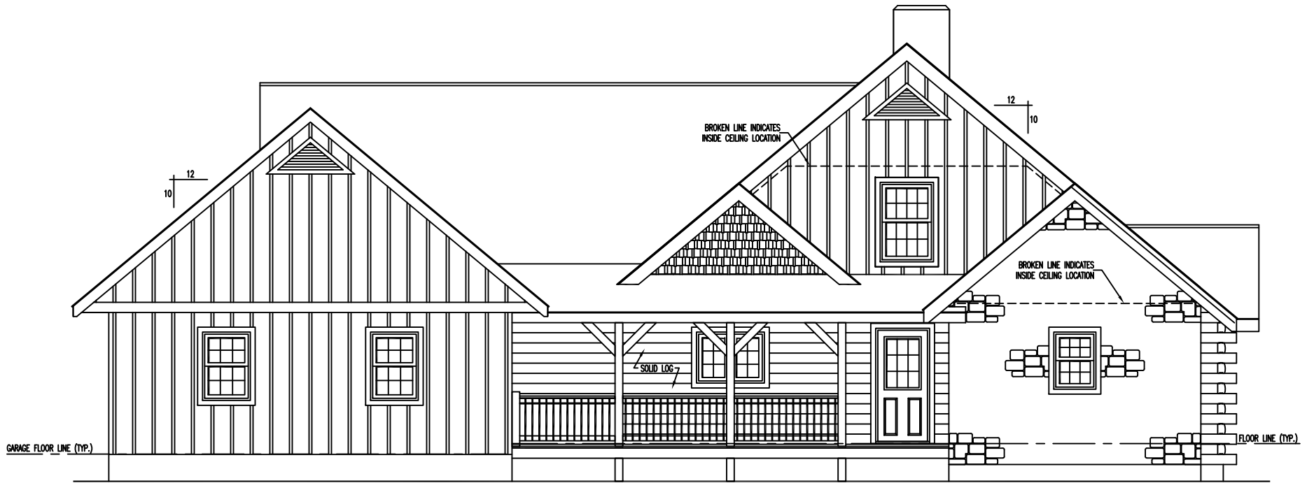
FRONT ELEVATION
