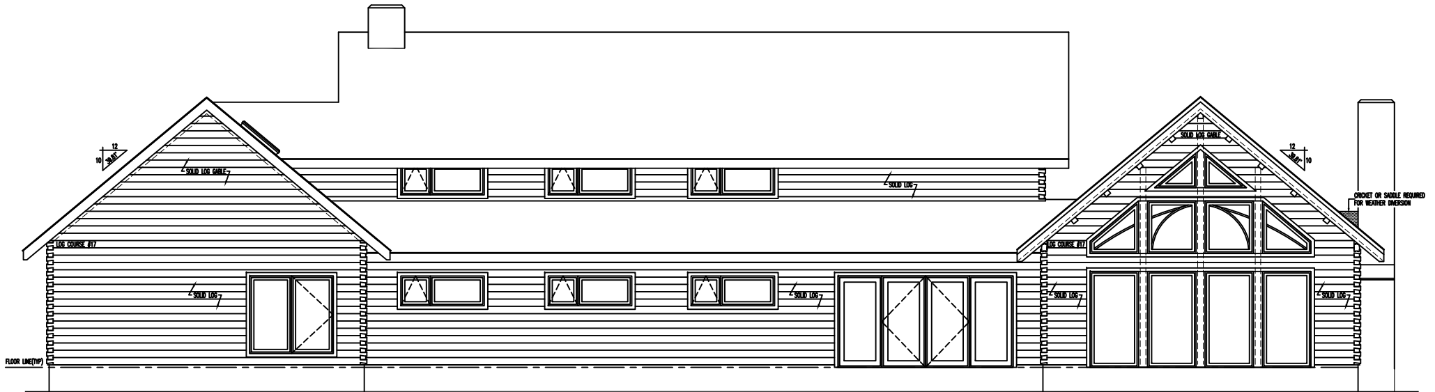
FRONT ELEVATION
