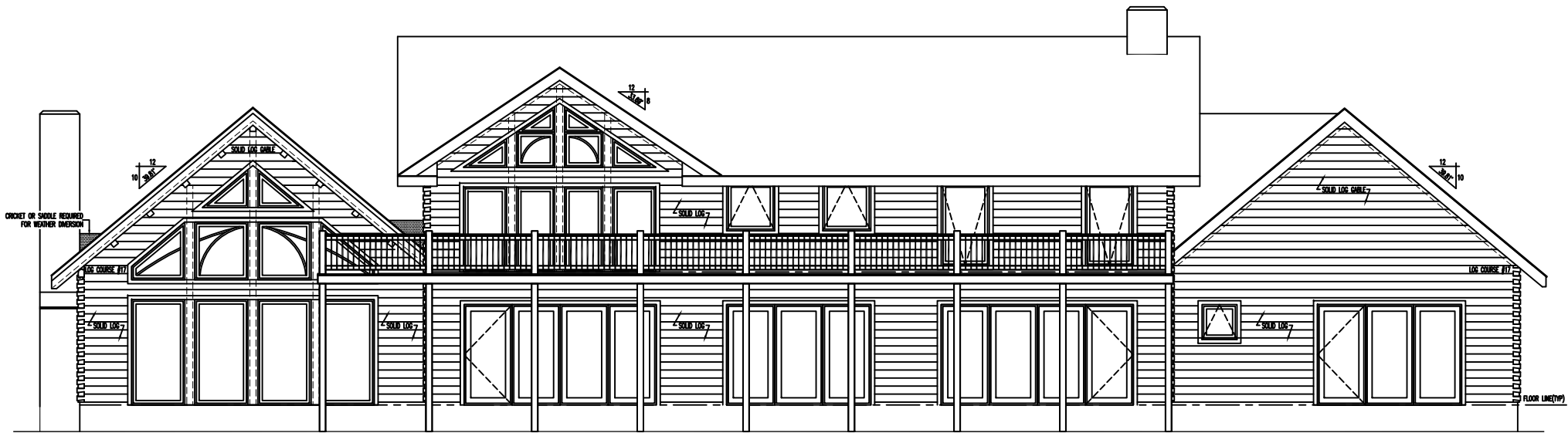
REAR ELEVATION
