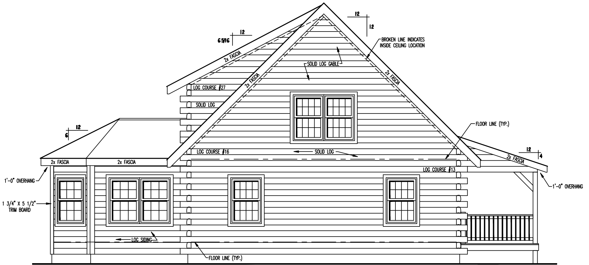
LEFT ELEVATION
