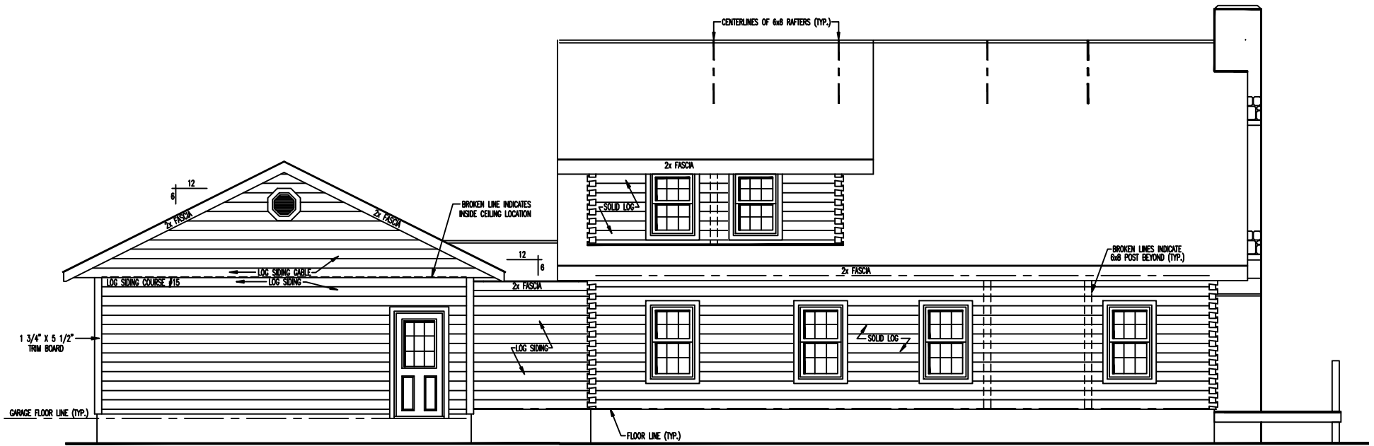
LEFT ELEVATION
