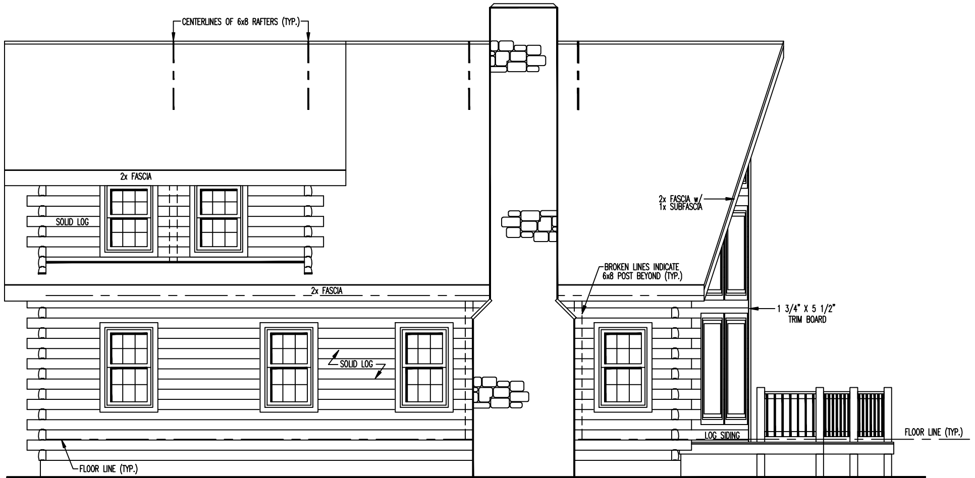
LEFT ELEVATION
