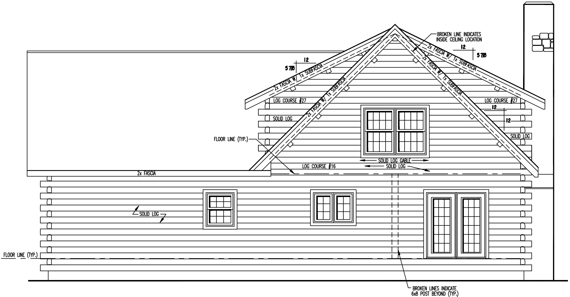
REAR ELEVATION
