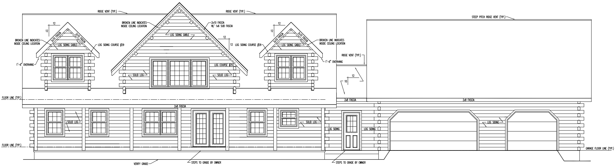
FRONT ELEVATION
