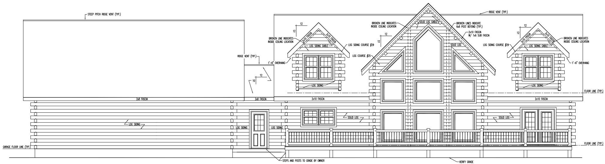
REAR ELEVATION
