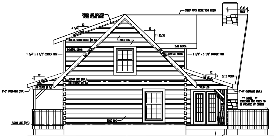
LEFT ELEVATION
