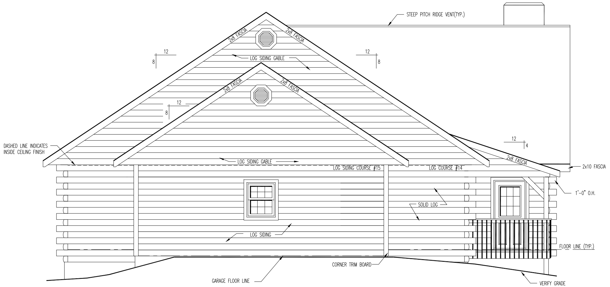
LEFT ELEVATION
