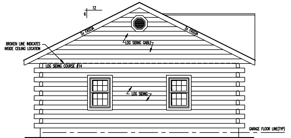
LEFT ELEVATION
