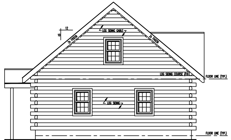
LEFT ELEVATION
