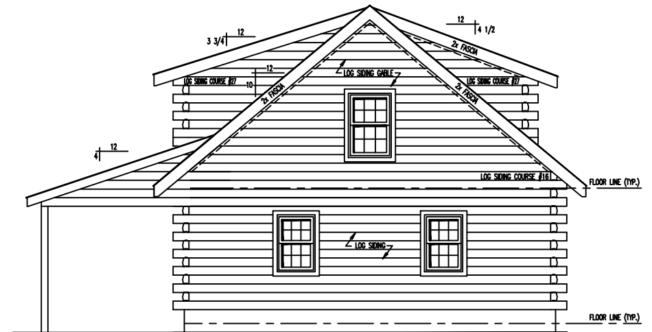
LEFT ELEVATION
