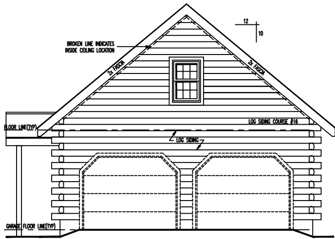
FRONT ELEVATION
