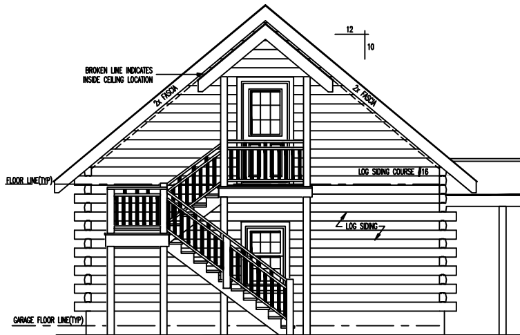
REAR ELEVATION
