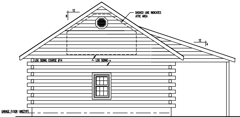
REAR ELEVATION
