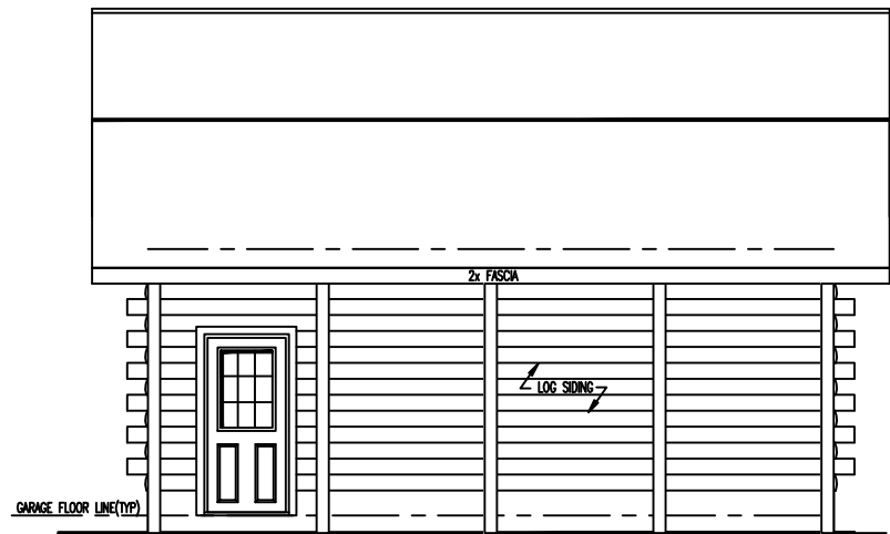
LEFT ELEVATION
